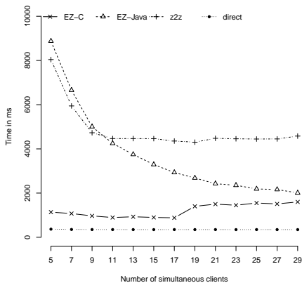
Fig. 3. Time to send 1000 message of 10kB by N clients.
