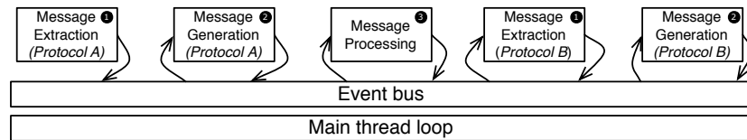
Fig. 2. Event-based processing chain
