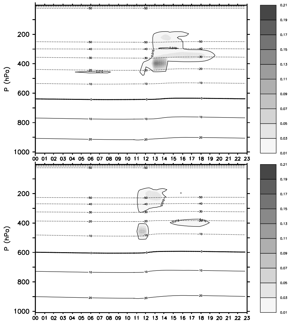
Figure 11. Diurnal cycle of the convective cloud ice content (shaded) (g/kg) and temperature of the environment (contoured) (°C) averaged over the equilibrium period for the (top) dry and the (bottom) wet cases. The additional contour line is the 0.01 g/kg isoline for q_{ice} .
