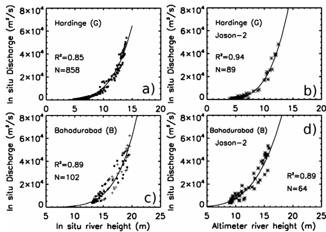
Figure 4. Rating curves (see text for details), i.e., the scatterplot showing the relationship between river height and river discharge. (a) Scatterplot ( H_G-Q_G ) for 858 measurements during 2006–2011 between in situ river height and in situ river discharge for the Ganga at Hardinge. (b) Scatterplot ( H_{J-2/G}-Q_G ) of in situ river discharge observations versus Jason-2 altimeter-based river height measurements for Hardinge, Ganga. (c) Scatterplot ( H_B-Q_B ) for 102 measurements during 2008–2011 between in situ river height and in situ river discharge for the Brahmaputra at Bahadurabad. Plus signs represent measurements made during the river height rising period and crosses represent measurements made during the river height decreasing period. (d) Scatterplot ( H_{J-2/B}-Q_B ) of in situ river discharge observations versus Jason-2 altimeter-based river height measurements for Bahadurabad, Brahmaputra. In each figure, the number of points ( N ) and the correlation coefficient ( R ) are indicated. The solid lines show the regression relation (power law function).
