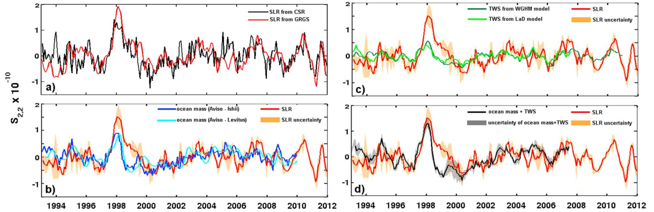
Figure 1. (a) S_{2,2} variations from SLR data computed by GRGS (red curve) and CSR (black curve). (b–d) S_{2,2} variations from SLR data (mean of CSR and GRGS solutions) are in red with uncertainty (orange shaded area). The ocean mass contribution is plotted on Figure 1b with estimations based on data from Levitus et al. [2012] (light blue curve) and from Ishii and Kimoto [2009] (dark blue curve). The land mass contribution is plotted on Figure 1c with estimations based on the LaD model (light green curve) and on the WGHM model (dark green curve). The sum of the ocean and land mass contributions is plotted on Figure 1d (black curve) with uncertainty (grey shaded area).
