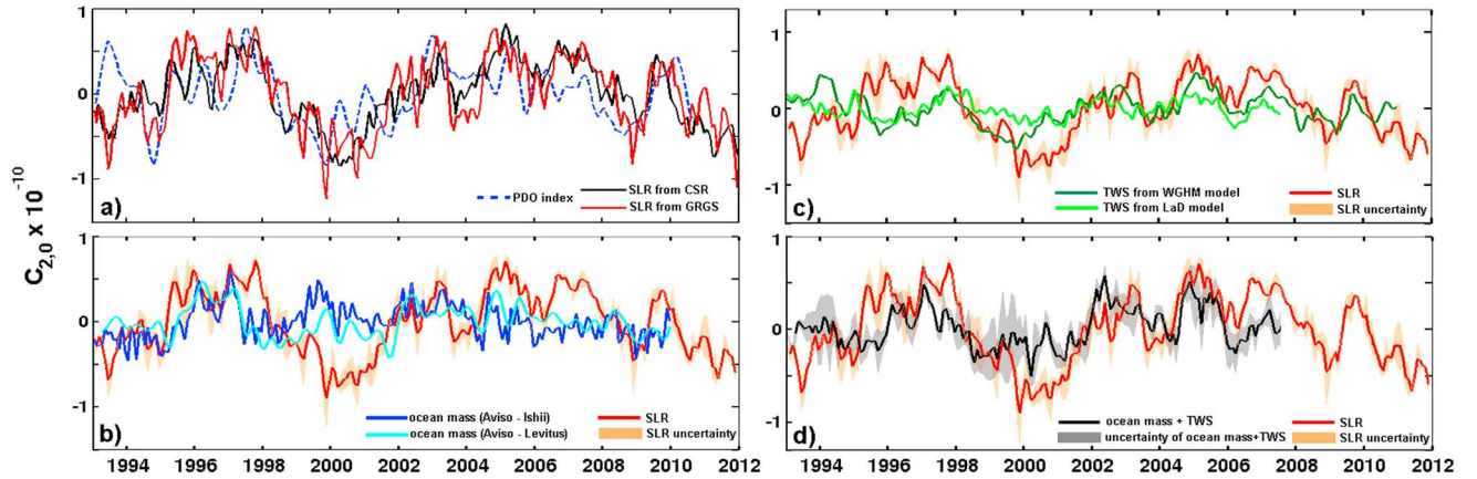
Figure 3. (a) C_{20} variations from SLR data computed by GRGS (red curve) and CSR (black curve) against the normalized PDO index (blue dashed curve). (b–d) C_{20} variations from SLR data (mean of CSR and GRGS solutions) are in red with uncertainty (orange shaded area). The ocean mass contribution is plotted on Figure 3b with estimations based on data from Levitus et al. [2012] (light blue curve) and from Ishii and Kimoto [2009] (dark blue curve). The land mass contribution is plotted on Figure 3c with estimations based on the LaD model (light green curve) and on the WGHM model (dark green curve). The sum of the ocean and land mass contributions to C_{20} is plotted on Figure 3d (black curve) with uncertainty (grey shaded area).
