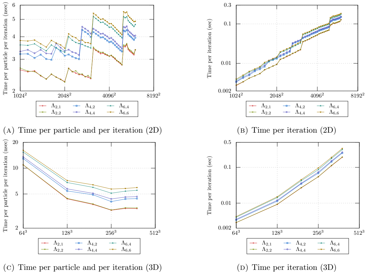
FIGURE 17. Overall performances for different problem sizes in double precision. (lower is better). Times are averaged over 20 independent executions.
