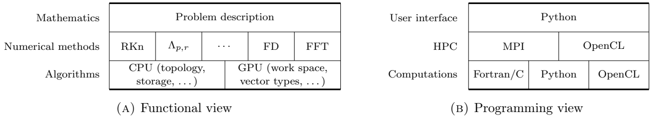
FIGURE 9. Application layout.
