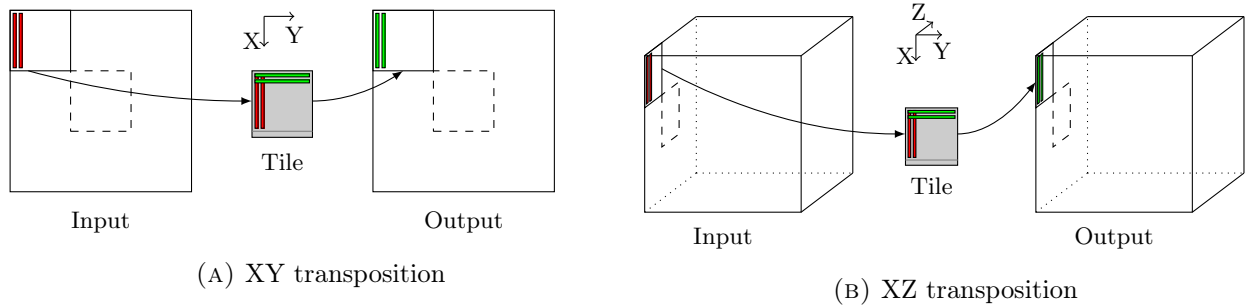
FIGURE 11. Transposition kernels.
