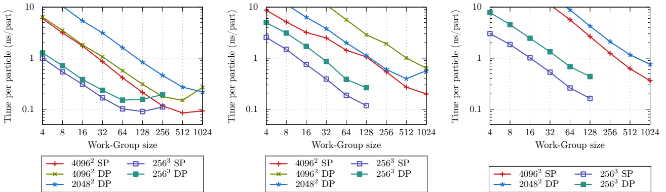
(A) Advection kernels (RK4) (B) Remeshing kernels ( \Lambda_{2,1} ) (C) Monolithic kernels (RK4 + \Lambda_{2,1} )
