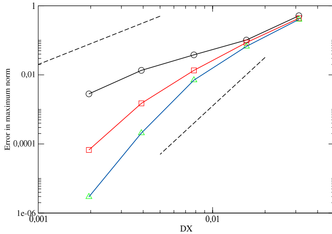
FIGURE 3. Refinement study for the 2D advection field (4.2). CFL value is equal to 12. Left picture : black-circle curve : kernel \Lambda_{2,1} ; red-square : kernel \Lambda_{4,2} ; blue-triangle : kernel \Lambda_{6,4} ; dashed lines indicate slopes corresponding to second and fourth order convergence. Right table: average order of convergence for these RPM.
