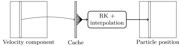
FIGURE 13. Advection algorithm.
