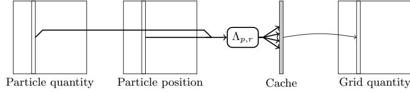
FIGURE 15. Remeshing algorithm.
