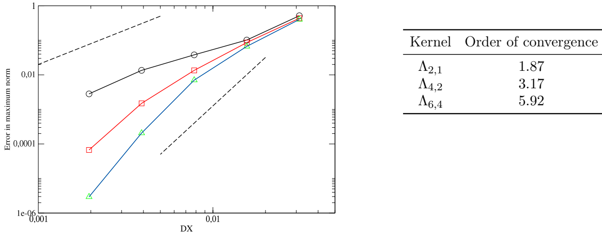
FIGURE 3. Refinement study for the 2D advection field (4.2). CFL value is equal to 12. Left picture : black-circle curve : kernel \Lambda_{2,1} ; red-square : kernel \Lambda_{4,2} ; blue-triangle : kernel \Lambda_{6,4} ; dashed lines indicate slopes corresponding to second and fourth order convergence. Right table: average order of convergence for these RPM.
