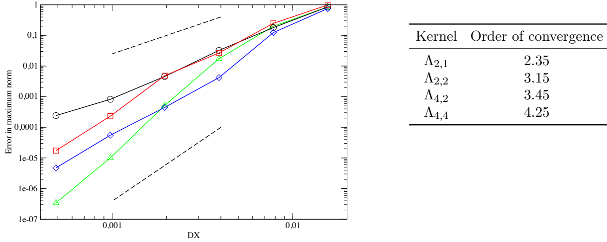
FIGURE 2. Refinement study for the 1D advection equation (4.1) and several first to fourth order RPM and CFL value equal to 12. Left picture : black-circle curve : kernel \Lambda_{2,1} ; red-square : kernel \Lambda_{2,2} ; blue-diamond : kernel \Lambda_{4,2} ; green-triangle : \Lambda_{4,4} ; dashed lines indicate slopes corresponding to second and fourth order convergence. Right table: average order of convergence for these RPM.
