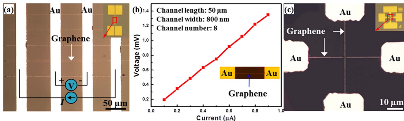
Figure 4 | Electrical characterization of graphene devices fabricated by the LDW method. (a) An optical micrograph of a four-terminal device for sheet resistance measurements. (b) I - V curve of the four-terminal electrical device with eight graphene straight line channels as shown in a, the inset show an optical micrograph of one graphene channel between two Au contacts. (c) An optical micrograph of an electrical device with (a) Greek-cross graphene pattern for Hall measurements. The insets in (a) and (c) show the zoomed-out optical micrographs of the parallel line and cross-bar graphene devices, respectively.
