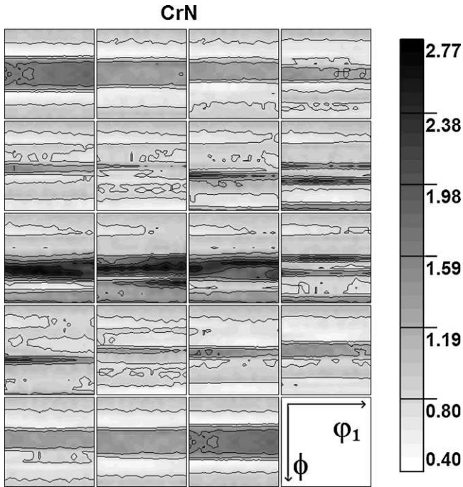
Fig. 10. Orientation distribution function (ODF) for CrN coating determined by X-ray diffraction. The sections through Euler space [\phi_1, \phi] with the step of 5^\circ along \phi_2 axis are presented.
