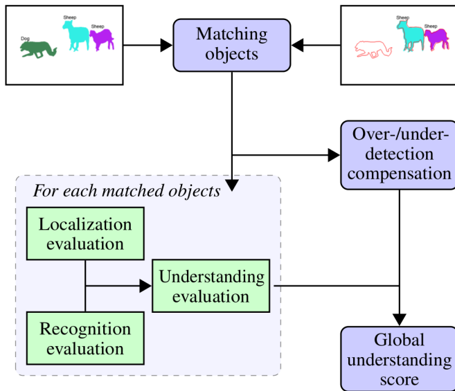
Figure 3: Image understanding metric
