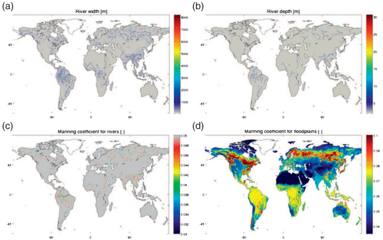
FIG. 4. Global distribution of HyMAP parameters at a 0.25^\circ spatial resolution: (a) river width derived from Eq. (13); (b) river depth derived from Eq. (14); (c) Manning roughness coefficient for rivers, as described by Eq. (15); and (d) Manning roughness coefficient for floodplains, Eq. (16).
