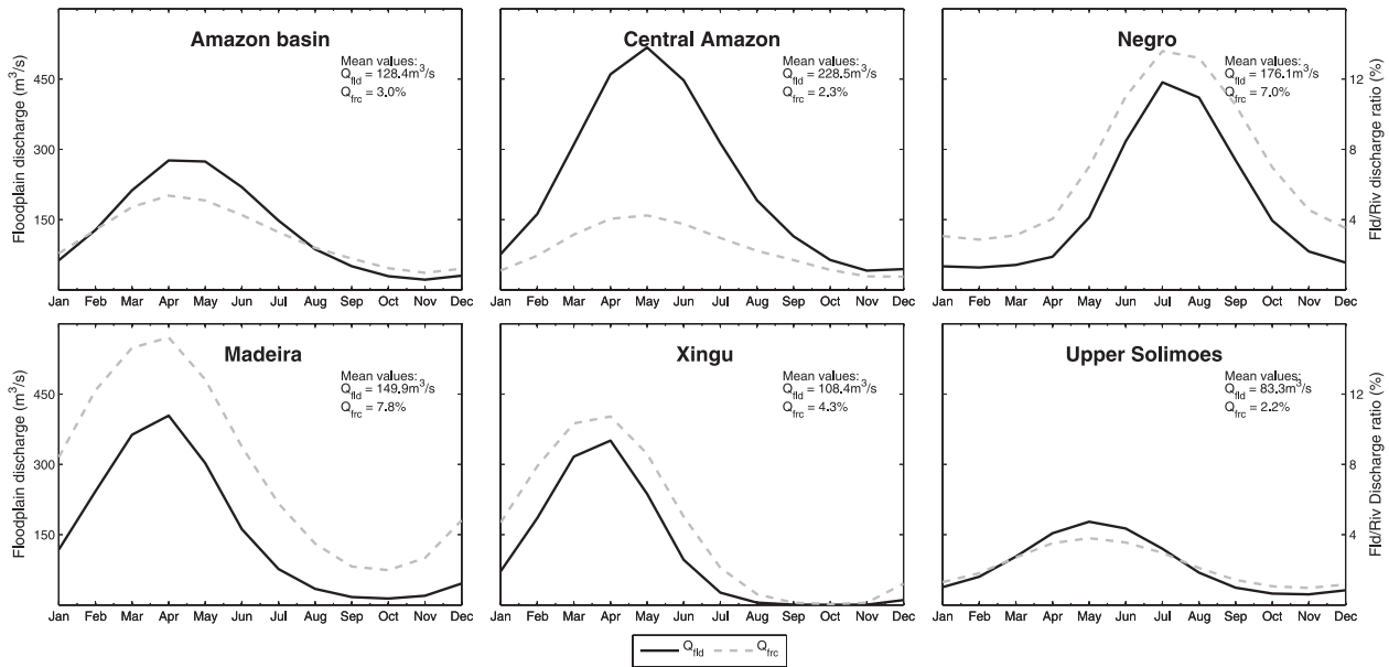
FIG. 14. Annual cycles of simulated floodplain water fluxes averaged for the Amazon basin and other five regions. Solid lines represent absolute water discharge discharges ( Q_{fld} ) in m^3 s^{-1} and dashed lines floodplain–river discharge fraction ( Q_{frc} ) in %.
