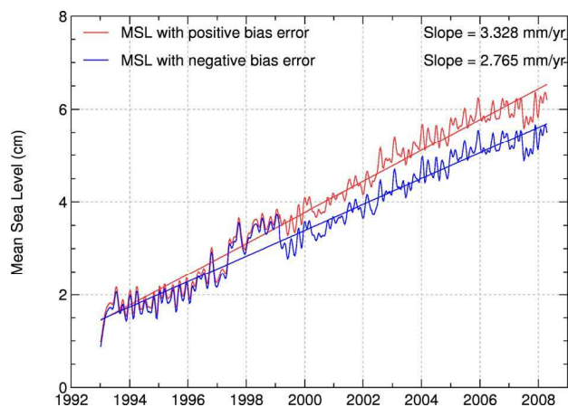
Fig. 6. Impact of the SSH bias uncertainty on the global MSL trend considering extreme SSH bias errors between TOPEX A and TOPEX B, and between TOPEX B and Jason-1.
