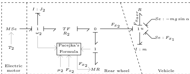
Fig. 3: Bond Graph model for control synthesis
