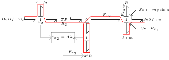
Fig. 5: Causal path on the bi-causal Bond Graph
