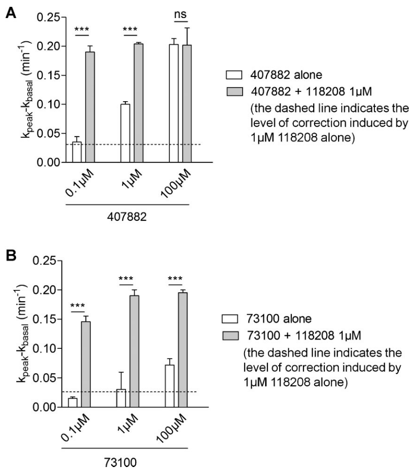
Figure 3. Synergistic effects of active compounds on iodide efflux in \Delta F508 -CFTR-expressing HeLa cells. The CFTR-dependent response was induced by co-treatment with 10 \mu\text{M} Fsk and 30 \mu\text{M} Gst.
