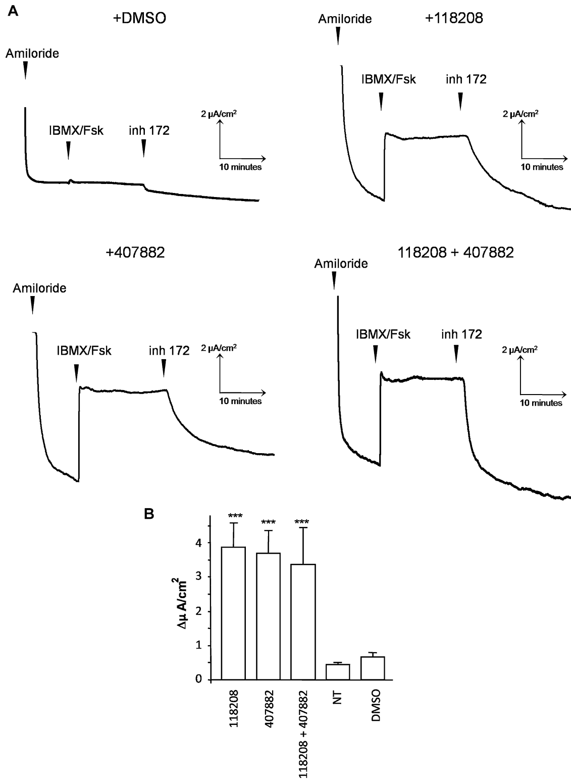
Figure 6. Rescue of \Delta F508 -CFTR function by compounds 407882 and 118208 in primary airway epithelial cells.
