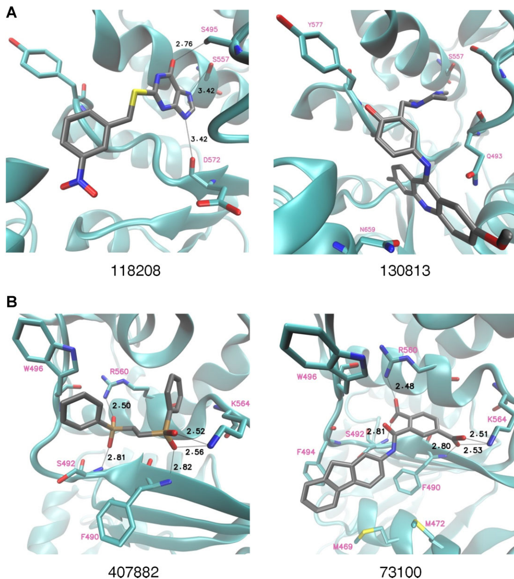
Figure 1. Binding modes for active correctors identified by VS. Potential hydrogen bonds are represented by black dashed lines. Distances in Angstroms (Å) are also listed. Essential residues are labelled.
