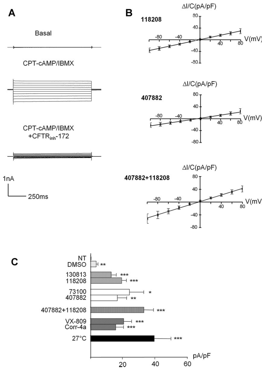
Figure 4. Effect of compounds on whole cell \text{Cl}^- currents recorded in HeLa cells by patch-clamp experiments.
