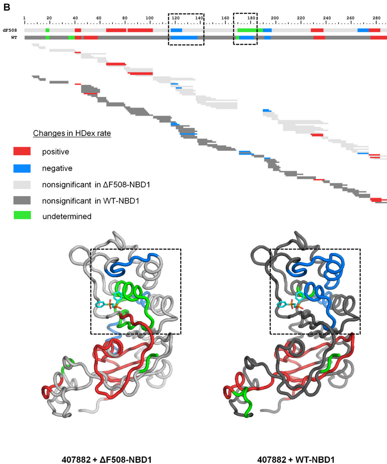
Figure 9. Effect of compounds 118208 and 407882 on \Delta F508 and WT-NBD1 structures tested by HDex-MS experiment. The coverage of \Delta F508 and WT-NBD1 sequences by peptic peptides has been shown on (upper panels). The peptides have also been mapped onto the \Delta F508-NBD1 structure – 'docking frame' (lower panels), and coincidences between localization of binding pockets for each molecule and peptides with diminished hydrogen-deuterium exchange rate have been indicated by dashed lines. Sequence coverage by peptic peptides was 94.5% for \Delta F508-NBD1 and 97.5%, for WT-NBD1.
