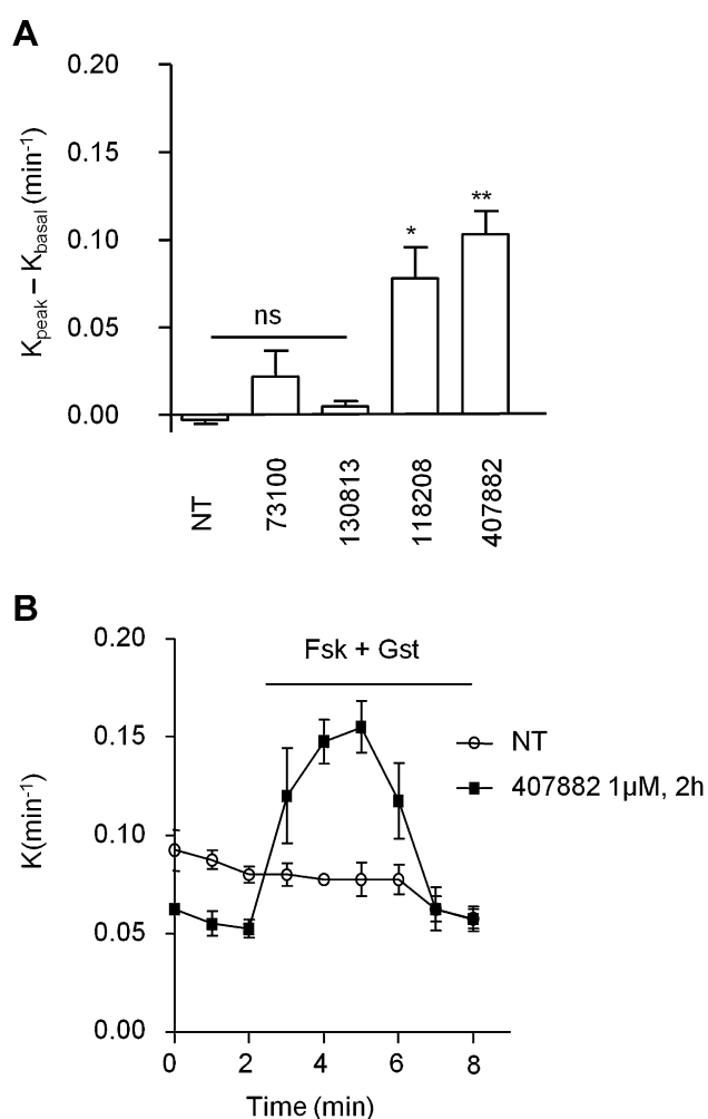
Figure 5. Iodide efflux in CF-KM4 cells.
