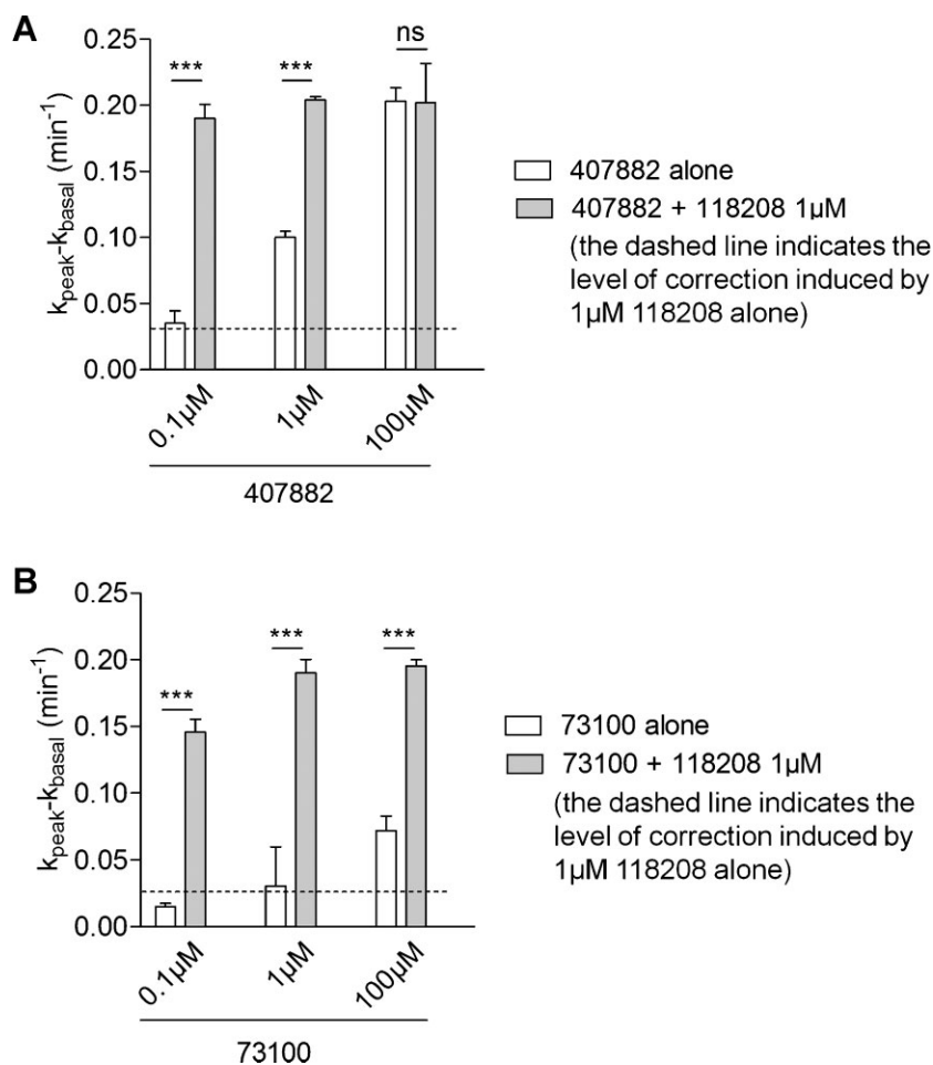
Figure 3. Synergistic effects of active compounds on iodide efflux in \Delta\text{F508} -CFTR-expressing HeLa cells. The CFTR-dependent response was induced by co-treatment with 10 \mu\text{M} Fsk and 30 \mu\text{M} Gst.
