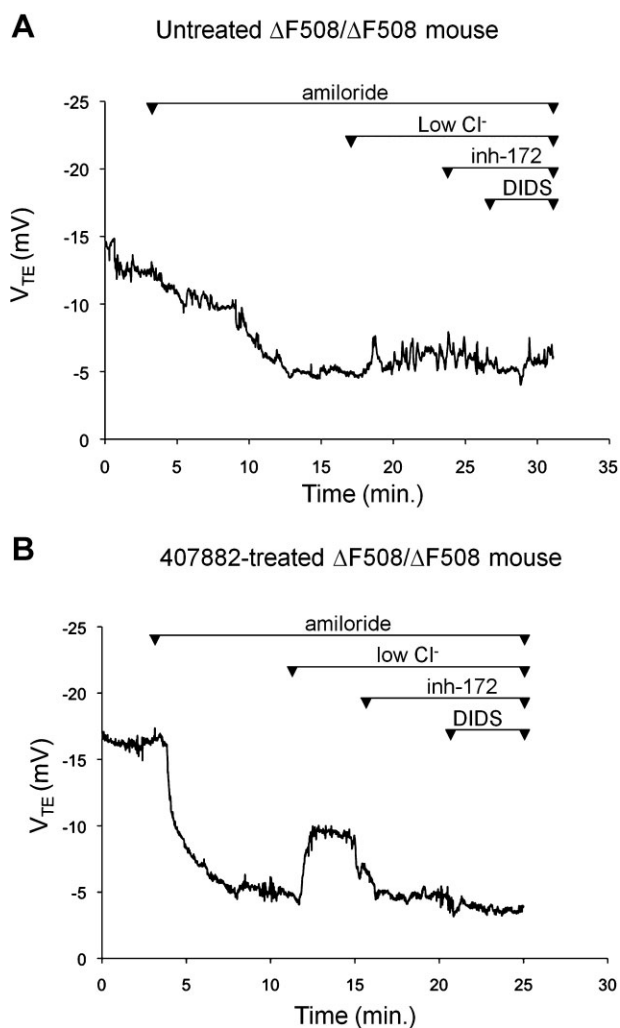
Figure 7. Effect of 407882 on nasal potential difference measurements in \Delta F508/\Delta F508 mice. Representative traces of nasal potential difference measurements in \Delta F508/\Delta F508 mice before and after treatment with 10 \mu\text{M} 407882 administered in nostril twice within 48 h. 100 \mu\text{M} amiloride-containing solution was applied to inhibit ENaC current, followed by a low \text{Cl}^- containing solution to unmask \text{Cl}^- secretion, and subsequently by 5 \mu\text{M} CFTR inh-172 and 100 \mu\text{M} of non-CFTR anion transport inhibitor, DIDS. A. Nasal potential ( V_{\text{TE}} ) changes recorded 7 days before the first administration of the compound (control). B. V_{\text{TE}} recorded 48 h after treatment of the same mouse with compound 407882.
