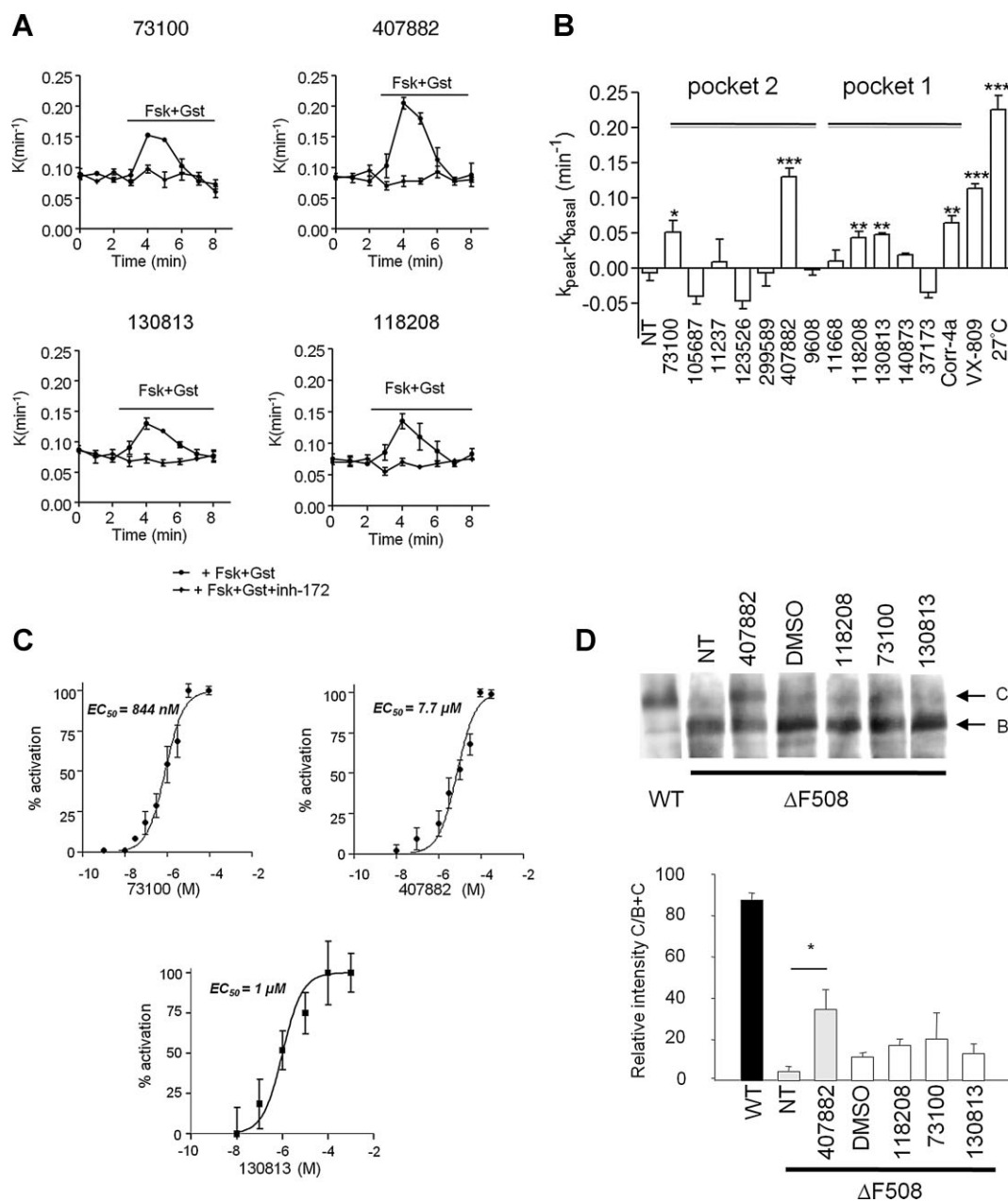
Figure 2. Effect of compounds on iodide efflux and CFTR maturation in \Delta F508-CFTR-expressing HeLa cells.
