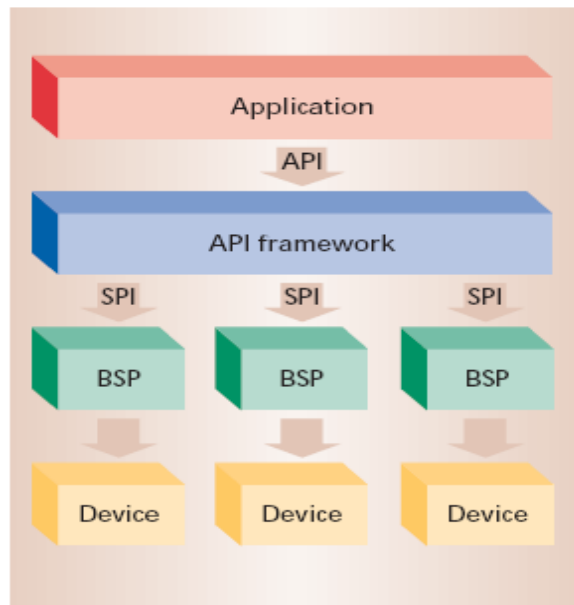
Figure 2: BioAPI components (source BioApi, 2005).
