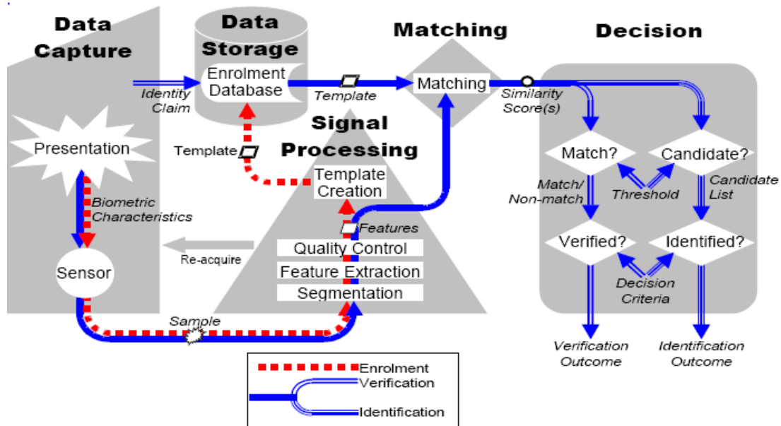
Figure 1: Diagram summarizing the various phases of a biometric system (Source: ISO/IEC JTC 1/SC 37 Part 1 Overview Standards Harmonization Document)
