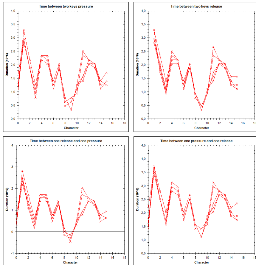
Figure 8: Plot of the biometric data for an individual for one session (5 acquisitions)
