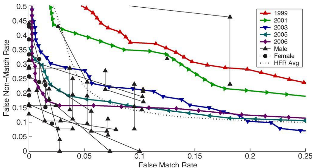
Figure 4: Example of DET curves used for the performance comparison of face recognition systems (source Adler et al., 2007).
