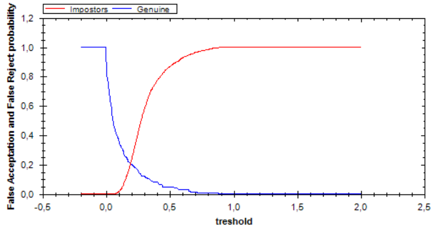
(a) Scores distribution
