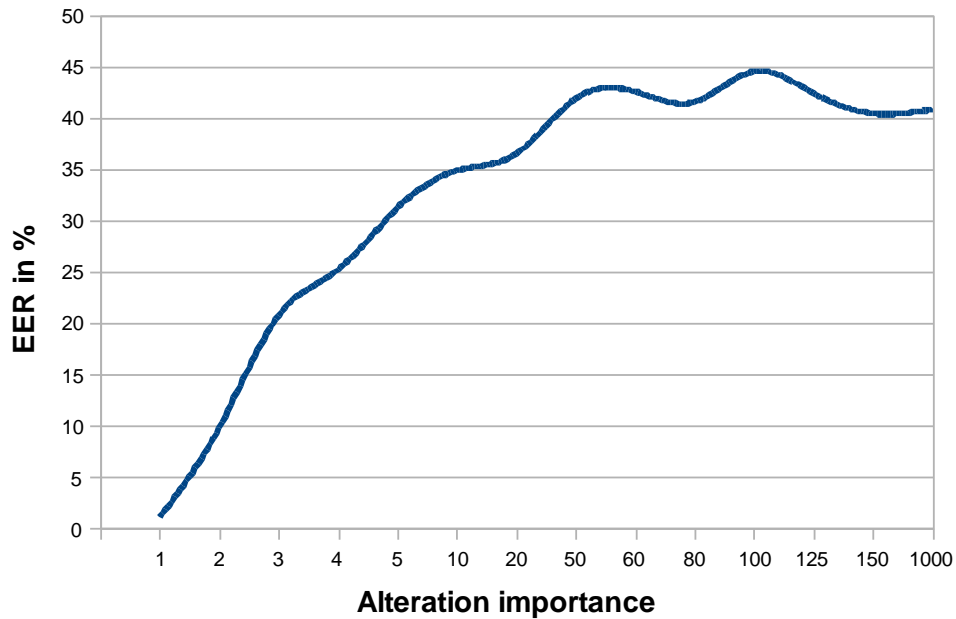
Figure 11: Evolution of the EER value given the amount of alterations.
