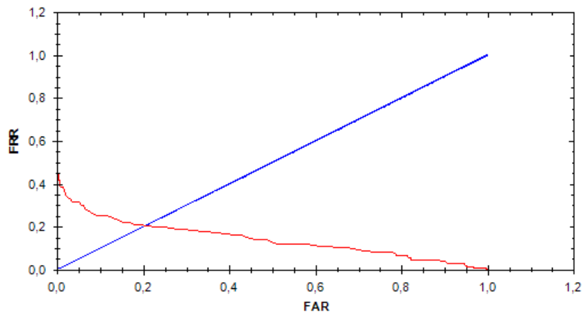
(b) Roc curve
