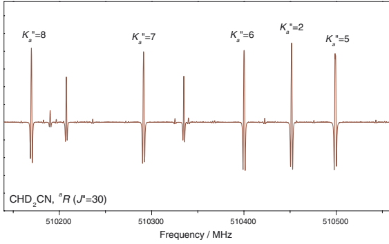
Fig. 1. Part of the submillimeter spectrum of CHD 2 CN.
