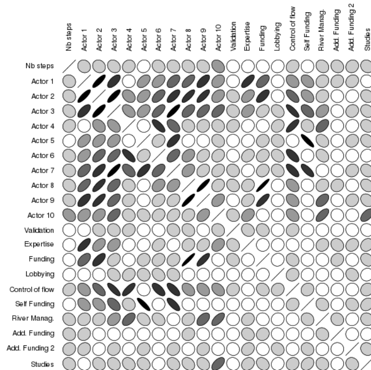
Figure 3. Graphical representation of the correlation coefficients between pairs of variables: the thinner the ellipse, the larger the absolute value of the correlation coefficient (see MURDOCH and CHOW, 1996, implemented in the R package ellipse). The grey level matches the absolute value of the correlation coefficient (darker colors are used for larger values).
