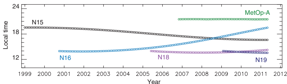
Figure 3. Equatorial crossing time (local) of temperature measurements for the AMSU instruments on board the different satellites for ascending orbits.
