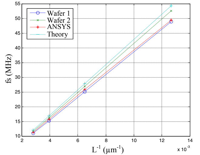
Figure 6: Resonance frequency as a function of resonator length.
