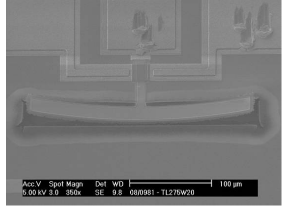
Figure 3: SEM view of a 75 \mu\text{m} length and 20 \mu\text{m} width TFEAR.
