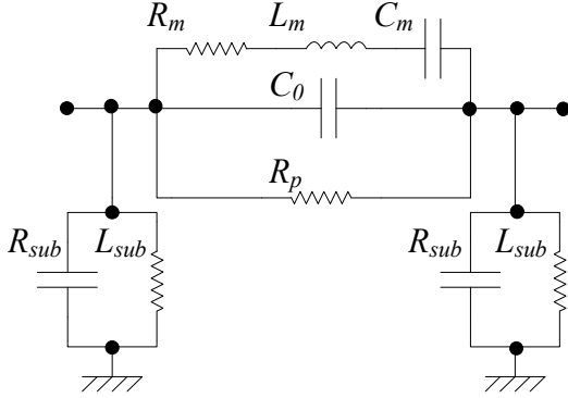
Figure 4: MBVD equivalent circuit of TFEAR.
