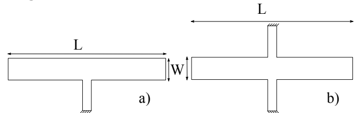
Figure 1: Schematic view of T-shaped (a) and X-shaped (b) TFEAR.
