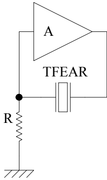
Figure 7: TFEAR based oscillator. Experimental values are: A=3 and R=680 \Omega .
