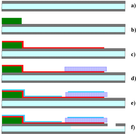
Figure 2: TFEAR cross section process flow views.
