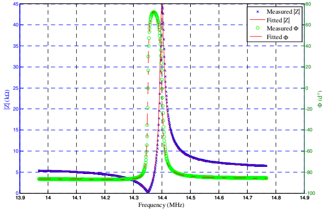
Figure 5: Examples of measured and fitted impedance amplitude and phase.
