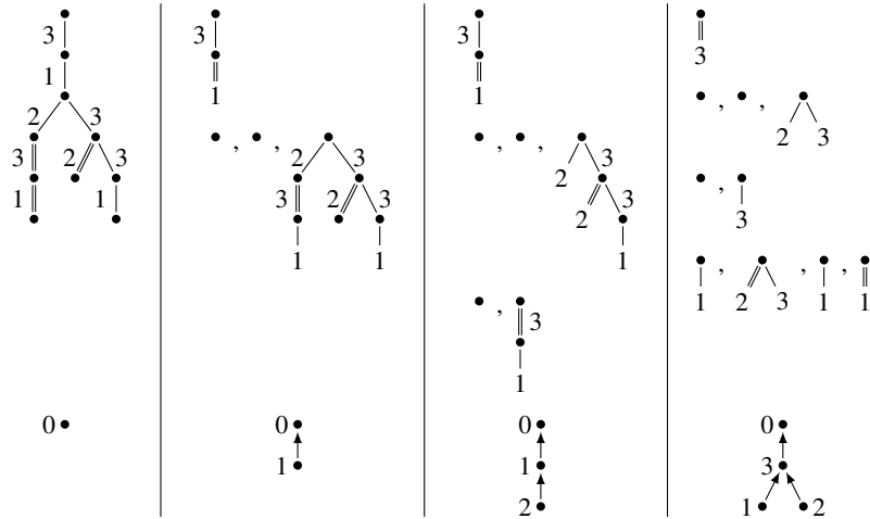
Fig. 1. An example with k = 3 , a tree of \mathcal{S}_0 and the corresponding elements of \mathcal{S}_1 , \mathcal{S}_2 and \mathcal{S}_3 (from left to right), with their associated Cayley trees (bottom). Marked edges are represented as double lines.
