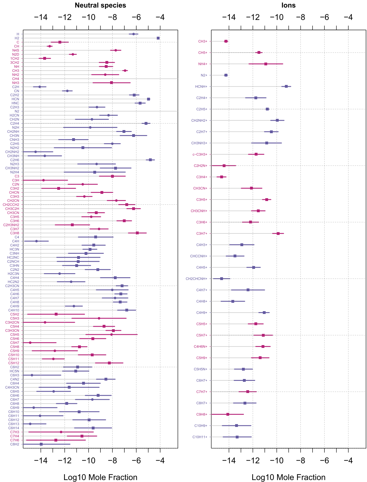
Fig. 3. Mole fractions (normalized to N 2 ) of neutral species (left panel) and ions (right panel) at the stationary state for the 500 runs of the 1-cell model with all uncertain parameters. The species are sorted downwards by increasing mass. Only species with an average mole fraction above 10 -15 are represented and CH 4 has been left out of the graph for legibility: its Log 10 Mole Fraction is -0.9545 \pm 0.0001 . Cx blocks are materialized by alternating colors. Neutral species with even/odd electron counts are marked by a square/circle symbol. Error bars cover a 95% confidence intervals.
