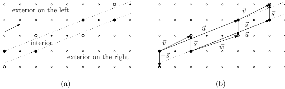
Fig. 2. The set of black disks lying between the two parallel dotted lines defines the DSL \mathcal{D}(2, 5, 0) . The large black and white disks depict the leaning (weakly interior) and Bezaout (weakly exterior) points of \mathcal{D} . In (b), vectors \vec{v} , \vec{w} and \vec{s} show that the Bezaout points are closely related to the leaning points
