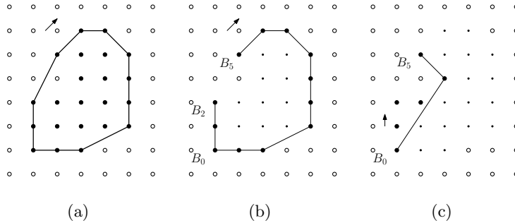
Fig. 3. In (a), the digital object depicted with black points is not convex because its convex hull contains one background point. In (b), the part (B_5B_2) is convex because there is no digital point between \overline{(B_5B_2)} and (B_5B_2) . Conversely, in (c), the part (B_0B_5) is concave because there is no digital point between \underline{(B_0B_5)} and (B_0B_5) .
