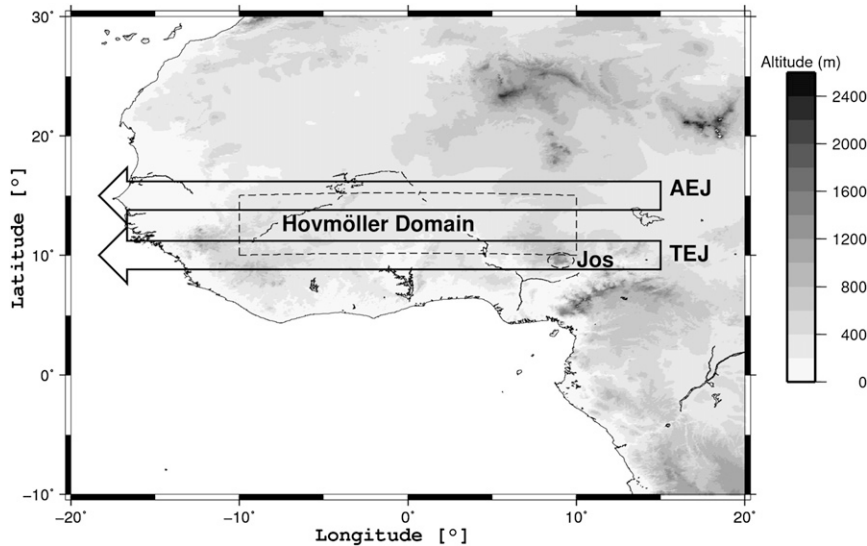
FIG. 1. West Africa with the study area ( 10^{\circ}\text{S} – 30^{\circ}\text{N} , 20^{\circ}\text{W} – 20^{\circ}\text{E} ) outlined. The gray shading indicates high terrain, and the Jos Plateau is indicated by a dashed ellipsis. Mean locations of TEJ and AEJ are highlighted by arrows. The domain of the systematic study is indicated by a dashed rectangle.
