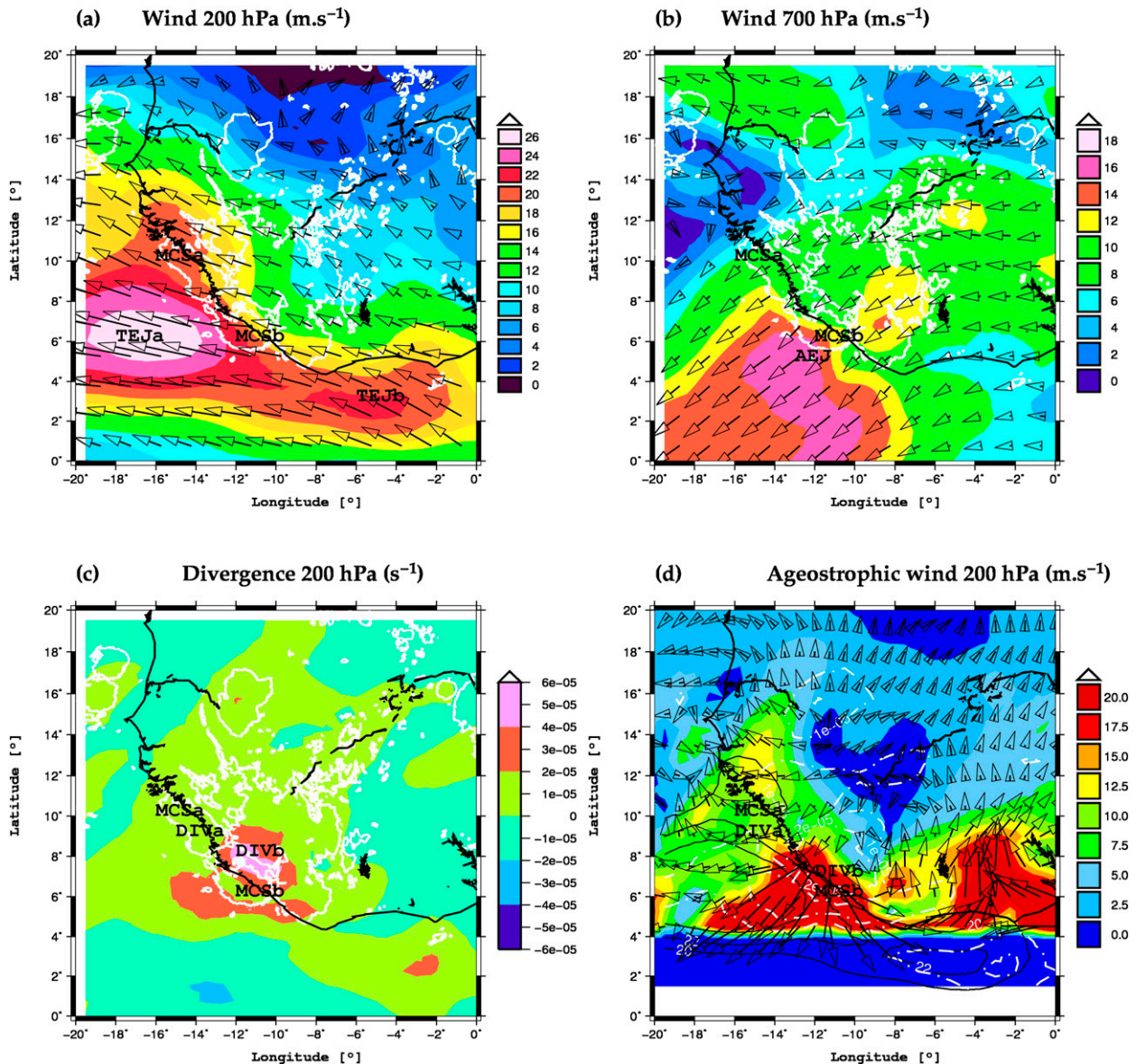
FIG. 6. Horizontal cross section of ECMWF fields at 0600 UTC 29 Jul 2006, the wind speed ( \text{m s}^{-1} ) (a) at 200 hPa and (b) at 700 hPa, (c) the divergence ( \text{s}^{-1} ) at 200 hPa, and (d) the ageostrophic wind estimation ( \text{m s}^{-1} ) at 200 hPa. The bold white solid line corresponds to the brightness temperature from MSG (K). The dotted–dashed white line in (d) corresponds to the positive area of divergence. Different dynamic entities are identified by MCS, TEJ, AEJ, and DIV. The thin black line indicates the West African coast and arrows indicate the wind direction. The ageostrophic wind is not calculated below 4^\circ of latitude.
