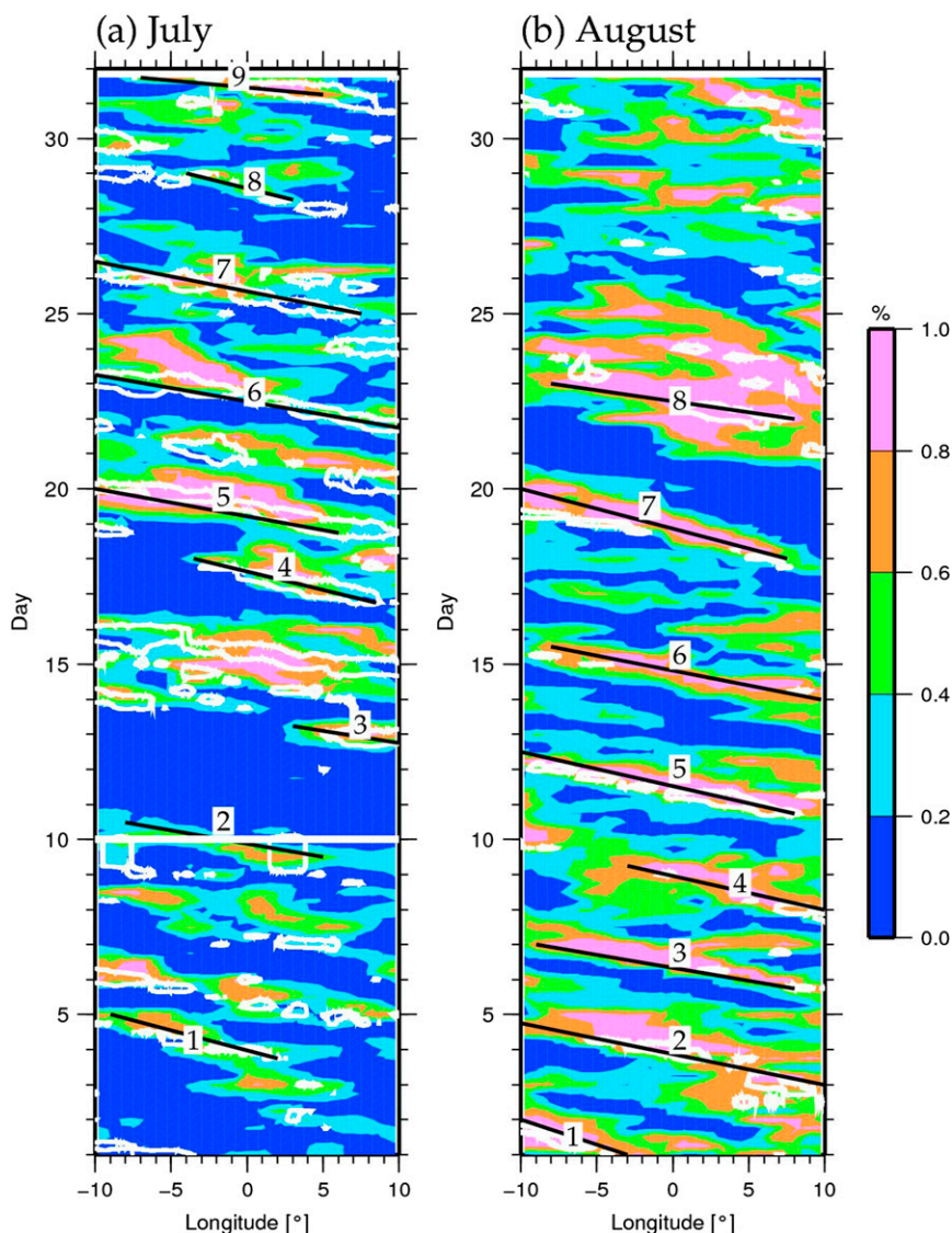
FIG. 8. Hovmöller diagrams on the high cloud cover from ECMWF (in color field) for (a) July and (b) August, averaged between 10^{\circ} and 15^{\circ} N (for July). The brightness temperature from MSG (253-K threshold) is indicated by the white contour. Solid white lines indicate the onset of the monsoon season. The solid black line corresponds to MCSs trajectories.
