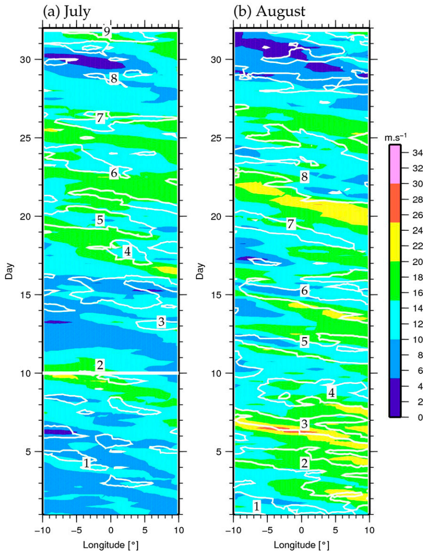
FIG. 9. Hovmöller diagrams on the wind speed at 200 hPa from ECMWF for (a) July and (b) August, averaged between 10° and 15°N. The high cloud cover from ECMWF is indicated by white contours. The white solid line represents the onset of the monsoon season. Numbers inside the cloud contour indicate the well-reproduced cloud systems observed by MSG in the ERA-Interim.
