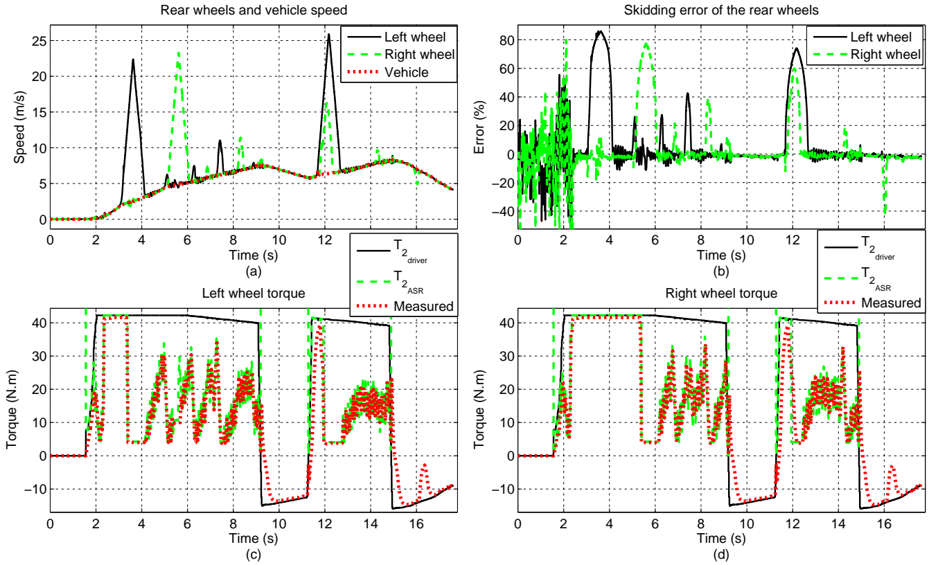
Fig. 9. Flat controller experimental results
