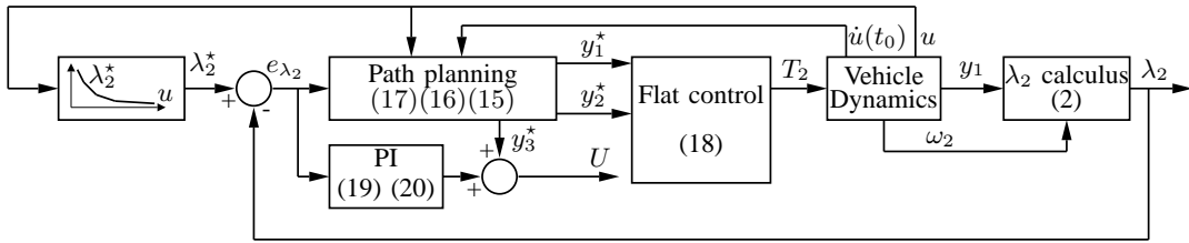
Fig. 6. Flat controller sketch
