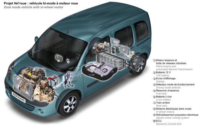
Fig. 1. VELROUE demonstrator vehicle
