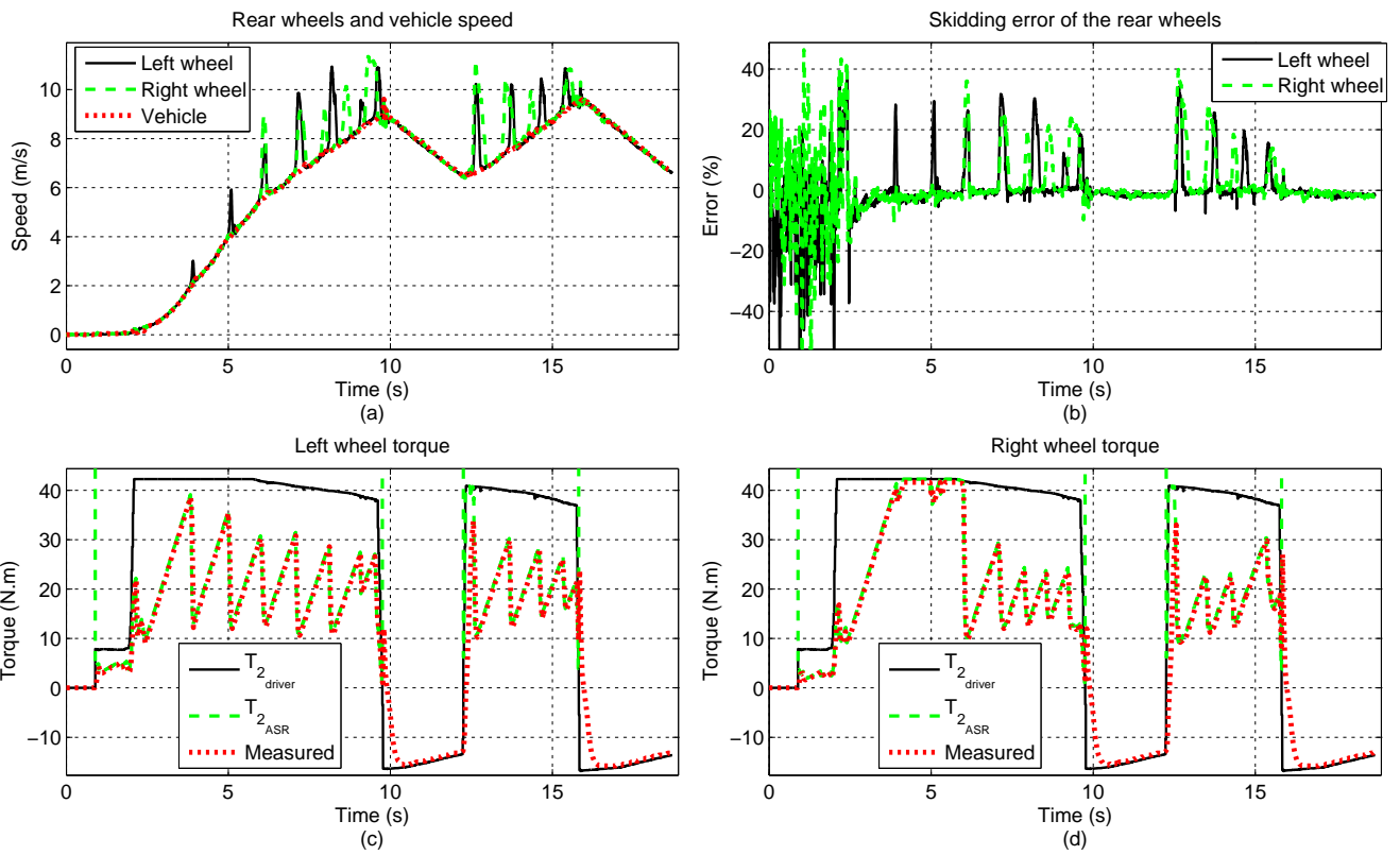
Fig. 7. PI controller experimental results
