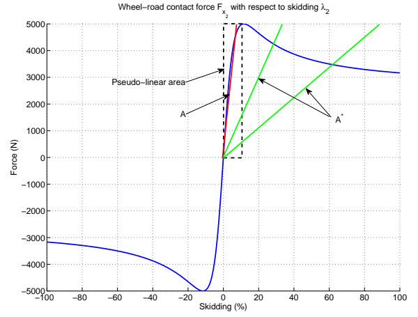
Fig. 5. Pseudo-linear area of Pacejka's representation
