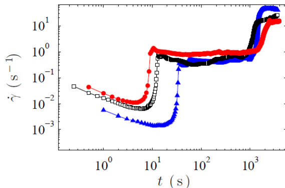
Figure 5: Shear rate responses \dot{\gamma}(t) for different CB gels under rough boundary conditions: C = 6\% w/w and \sigma = 13 Pa ( \blacktriangle ), C = 8\% w/w and \sigma = 45 Pa ( \square ), and C = 10\% w/w and \sigma = 90 Pa ( \bullet ). The imposed shear stresses were chosen so as to yield roughly the same failure times.
