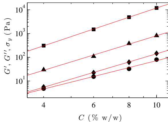
Figure 3: Rheological parameters gathered in Table I and plotted against the concentration C . Storage modulus G' (■) and loss modulus G'' (▲) measured at f = 1 Hz and \sigma = 2 Pa. Yield stress \sigma_{y1} inferred from the crossing between G' and G'' in an oscillatory stress sweep at f = 1 Hz (●). Yield stress \sigma_{y2} (◆) inferred from the Herschel-Bulkley fits of the flow curves shown in Fig. 2. Red lines are the best power-law fits whose exponents are given in the last line of Table I.
