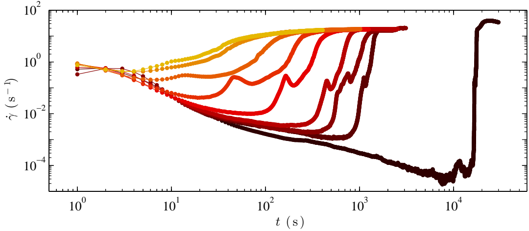
Figure 10: Creep experiments in an 8% w/w CB gel under smooth boundary conditions. Shear rate responses \dot{\gamma}(t) for different shear stresses \sigma applied at time t = 0 : from right to left, \sigma = 45, 50, 52, 53, 55, 60, 65, 70 , and 75 Pa.
