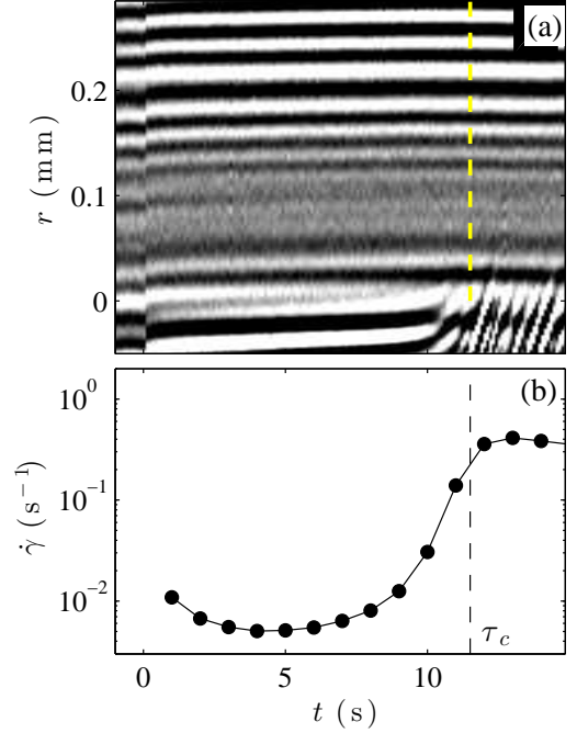
Figure 13: Creep regime for a 6% w/w CB gel at \sigma = 15 Pa under rough boundary conditions. (a) Spatiotemporal diagram of the pressure signal plotted as a function of the radial position r from the rotor (vertical axis) and time t (horizontal axis) after shear is started at t = 0 . Negative values of r correspond to locations inside the Plexiglas rotor. (b) Corresponding shear rate response \dot{\gamma}(t) . The dashed lines indicate the end of the creep regime at \tau_c \simeq 11.5 s which is seen to correspond to wall slip at the rotor.
