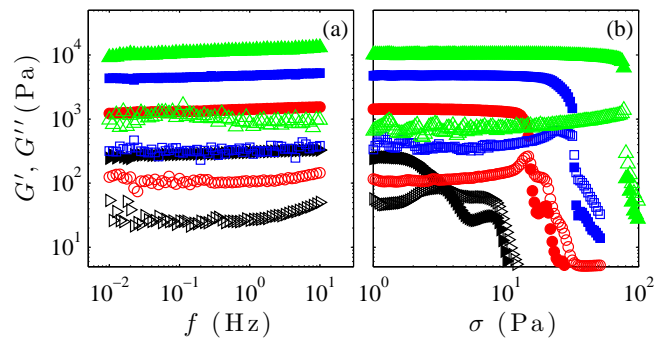
Figure 1: Viscoelastic moduli G' (filled symbols) and G'' (open symbols) of carbon black gels at C = 4 ( \triangleright ), 6 ( \circ ), 8 ( \square ), and 10\% w/w ( \triangle ) in a rough Couette geometry. (a) Frequency sweeps at a fixed stress amplitude \sigma = 2 \text{ Pa} . The waiting time per point is 6 oscillation periods. (b) Stress sweeps at a fixed frequency f = 1 \text{ Hz} with a waiting time of 5 s per point.
