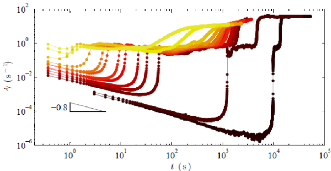
Figure 4: Creep experiments in an 8% w/w CB gel under rough boundary conditions. Shear rate responses \dot{\gamma}(t) for different shear stresses \sigma applied at time t = 0 : from right to left, \sigma = 24, 27, 35, 38, 41, 45, 47, 50, 52, 55, 60, 70, and 80 Pa.
