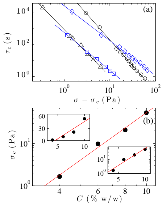
Figure 8: (a) Duration of the creep regime \tau_c vs \sigma for different CB gels under rough boundary conditions: C = 4 ( \Delta ), 6 ( \square ), 8 ( \circ ), and 10% w/w ( \diamond ) from left to right. Solid lines show the best power-law fits \tau_c \sim (\sigma - \sigma_c)^{-\beta} . The exponents \beta are given in Table II. (b) Fit parameter \sigma_c as a function of the gel concentration C in logarithmic scales. The red line is the power law \sigma_c \sim C^{3.7} . Top (bottom resp.) inset: same data as in the main figure but plotted in linear (semilogarithmic resp.) scales together with the best linear (exponential resp.) fit in red solid line.
