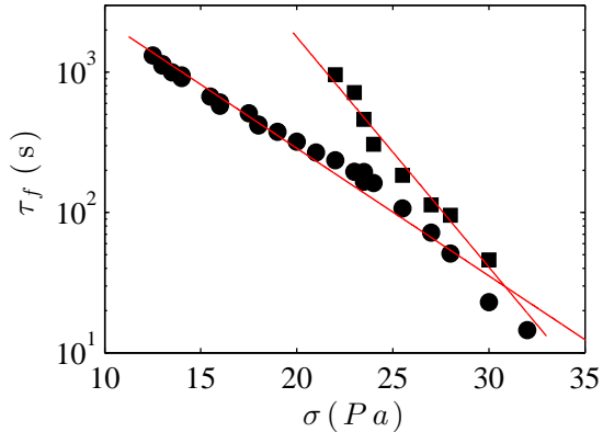
Figure 4: Fluidization time \tau_f after two different preshear protocols for a 6% w/w CB gel under rough boundary conditions: preshear for 20 s at +1000 s^{-1} (■) and at -1000 s^{-1} (●). The shear stress \sigma is applied in the positive direction once viscoelastic moduli have been measured for 300 s after preshear. Red lines are the best exponential fits \tau_f = \tau_0 \exp(-\sigma/\sigma_0) .
