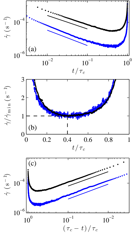
Figure 14: Initial creep regimes in two different CB gels already shown in Figs. 7 and 6. Black symbols correspond to the 8% w/w gel at \sigma = 27 Pa with \tau_c = 1216 s and blue symbols correspond to the 10% w/w gel at \sigma = 55 Pa with \tau_c = 11575 s. (a) \dot{\gamma} vs t/\tau_c in logarithmic scales showing the primary (Andrade) creep regime. Solid lines show the best power-law fits (shifted vertically for clarity) for 0.01 < t/\tau_c < 0.1 with exponents -0.81 (top) and -0.93 (bottom). (b) \dot{\gamma}/\dot{\gamma}_{\min} vs t/\tau_c in linear scales, where \dot{\gamma}_{\min} is an estimate of the minimum value reached by \dot{\gamma} . The vertical dashed line shows \tau_{\min} = 0.4\tau_c . (c) \dot{\gamma} vs (\tau_c - t)/\tau_c in logarithmic scales (with reverse horizontal axis) showing the tertiary creep regime prior to failure at the inner wall. Solid lines show the best power-law fits (shifted vertically for clarity) for 0.01 < (\tau_c - t)/\tau_c < 0.1 with exponents -0.97 (top) and -1.0 (bottom).
