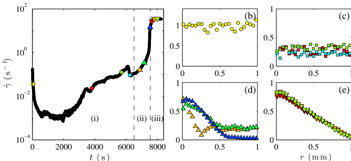
Figure 5: Creep experiment in a 6% w/w CB gel at \sigma = 16 Pa under smooth boundary conditions. (a) Shear rate response \dot{\gamma}(t) . The vertical dashed lines indicate the limits of the three regimes discussed in the text. The coloured symbols show the times at which the velocity profiles in (b)–(e) are recorded. Velocity profiles v(r, t_0) , where r is the distance to the rotor, normalized by the current rotor velocity v_0(t_0) at (b) t_0 = 39 s, (c) t_0 = 3806, 5700 , and 6240 s, (d) t_0 = 6871, 7157 , and 7536 s, and (e) t_0 = 7650, 7800 , and 8000 s.
