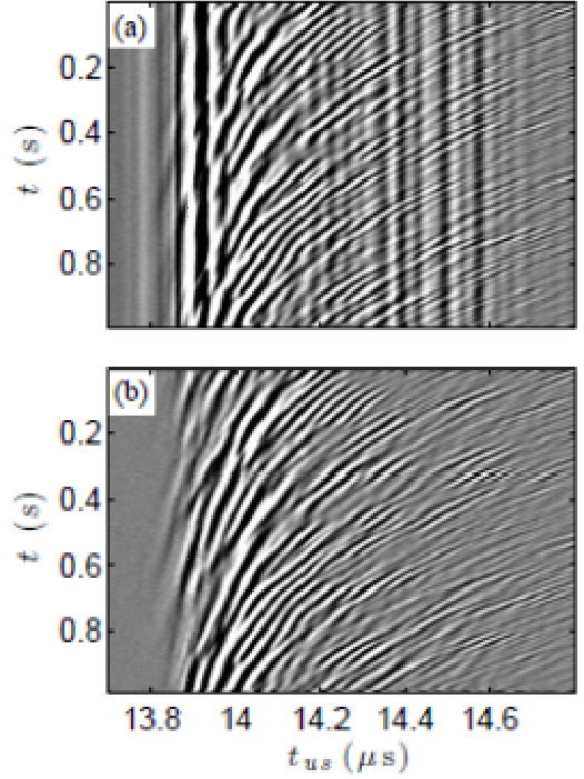
Figure 2: Spatiotemporal diagrams of the pressure signal recorded as a function of time t_{us} (horizontal axis) after a single pulse is sent at time t (vertical axis). (a) Raw data. (b) Same data after fixed echoes have been removed following the procedure described in the text. The pressure signal is coded in linear gray levels.
