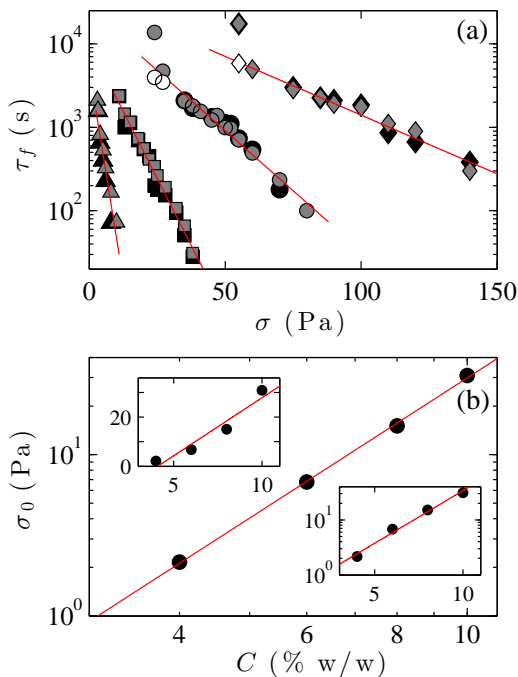
Figure 9: (a) Fluidization time \tau_f vs \sigma for different CB gels under rough boundary conditions: C = 4 ( \Delta ), 6 ( \square ), 8 ( \circ ), and 10% w/w ( \diamond ) from left to right. Gray symbols correspond to estimations derived from rheological data while black symbols are times extracted from velocity measurements. The red lines are the best exponential fits \tau_f = \tau_0 \exp(-\sigma/\sigma_0) when excluding stresses where \tau_c > 0.2\tau_f (the three corresponding points are indicated by showing \tau_f - \tau_c in white symbols). (b) Fit parameter \sigma_0 as a function of the gel concentration C in logarithmic scales. The red line is the power law \sigma_0 \sim C^{2.9} . Top (bottom resp.) inset: same data as in the main figure but plotted in linear (semilogarithmic resp.) scales together with the best linear (exponential resp.) fit in red solid line.
