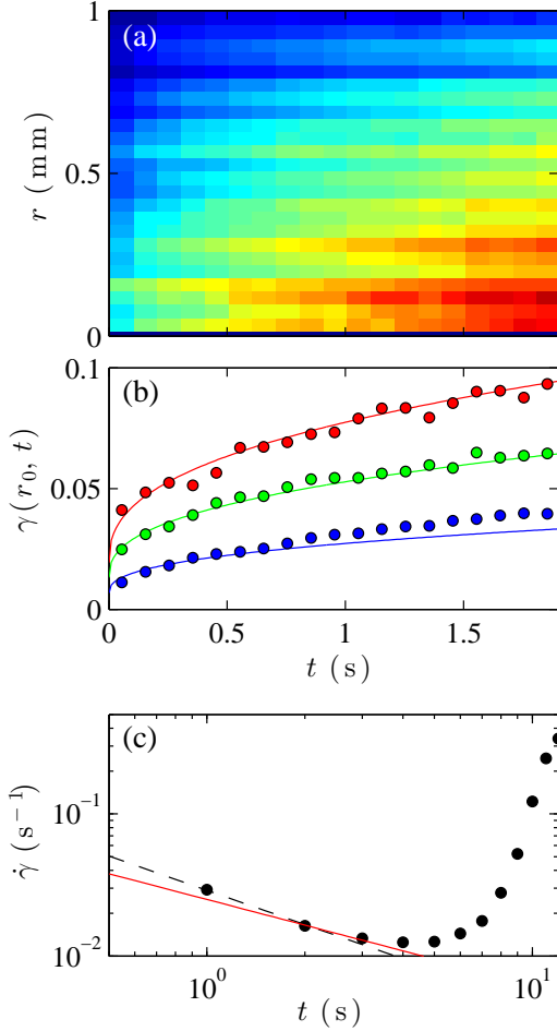
Figure 12: Creep regime for a 6% w/w CB gel at \sigma = 17 Pa under rough boundary conditions. (a) Spatiotemporal diagram of the local strain \gamma(r, t) coded in linear color levels. Blue corresponds to 0 and red to a strain of 0.1. (b) Local strain \gamma versus time t at various locations within the gap: r_0 = 0.12 (top red symbols), 0.40 (middle green symbols), and 0.69 mm (bottom blue symbols). The solid lines are \gamma(r_0, t) = (\gamma_0 + \lambda t^{0.4}) \cdot (1 - r_0/e) with \gamma_0 = 2.2 % and \lambda = 0.066 . (c) Global shear rate response \dot{\gamma}(t) recorded simultaneously by the rheometer. The black dotted line and the red solid line are power laws with exponents -0.8 and -0.6 respectively.
