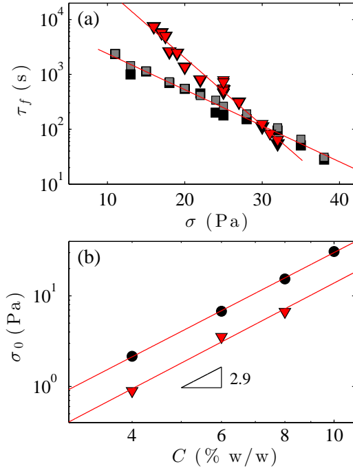
Figure 11: (a) Fluidization time \tau_f vs \sigma for a 6% w/w CB gel under rough ( \square ) and smooth ( \nabla ) boundary conditions. Gray and red symbols correspond to estimations derived from rheological data while black symbols are times extracted from velocity measurements. Red lines are the best exponential fits \tau_f = \tau_0 \exp(-\sigma/\sigma_0) . (b) Fit parameter \sigma_0 as a function of the gel concentration C in rough ( \bullet ) and smooth ( \nabla ) boundary conditions. Red lines are power laws \sigma_0 \sim C^{2.9} .
