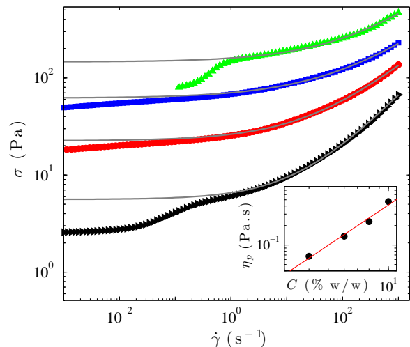
Figure 2: Flow curves \sigma vs \dot{\gamma} of carbon black gels at C = 4, 6, 8, and 10\% w/w from bottom to top, in a rough Couette geometry. The shear rate is swept down from \dot{\gamma} = 10^3 \text{ s}^{-1} with a logarithmic spacing of 15 points per decade and a waiting time of 1 s per point. Solid lines are fits using a Herschel-Bulkley law, \sigma = \sigma_{y2} + A\dot{\gamma}^n , for \dot{\gamma} > 1 \text{ s}^{-1} . For C = 10\% w/w, shear rates smaller than 0.1 \text{ s}^{-1} could not be reached with such a short waiting time per point. Inset: viscosity \eta_p measured at the highest shear rate \dot{\gamma}_p = 10^3 \text{ s}^{-1} as a function of the gel concentration C . The red line is the best power-law fit which yields an exponent of 2.1.
