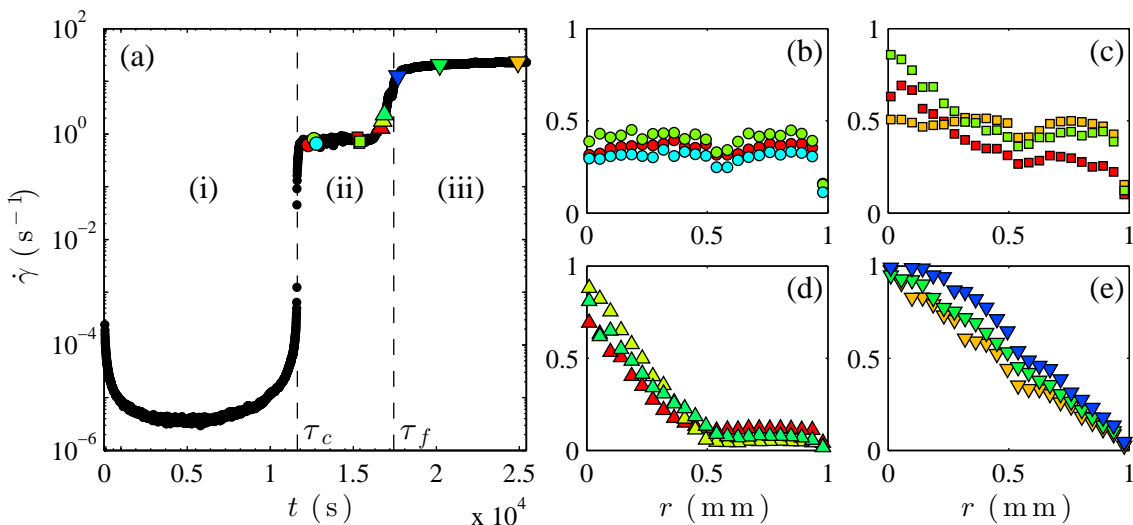
Figure 6: Creep experiment in a 10% w/w CB gel at \sigma = 55 Pa under rough boundary conditions. (a) Shear rate response \dot{\gamma}(t) . The vertical dashed lines indicate the limits of the three regimes discussed in the text, i.e. the end of the initial creep at \tau_c = 11630 s and the end of the fluidization regime at \tau_f = 17440 s. The coloured symbols show the times at which the velocity profiles in (b)–(e) are recorded. Shown in the right panel are individual velocity profiles v(r, t_0) , where r is the distance to the rotor, normalized by the current rotor velocity v_0(t_0) at (b) t_0 = 12278, 12630, and 12780 s, (c) t_0 = 15258, 15358, and 15401 s, (d) t_0 = 16642, 16773, and 16882 s, and (e) t_0 = 17696, 20204, and 24919 s.
