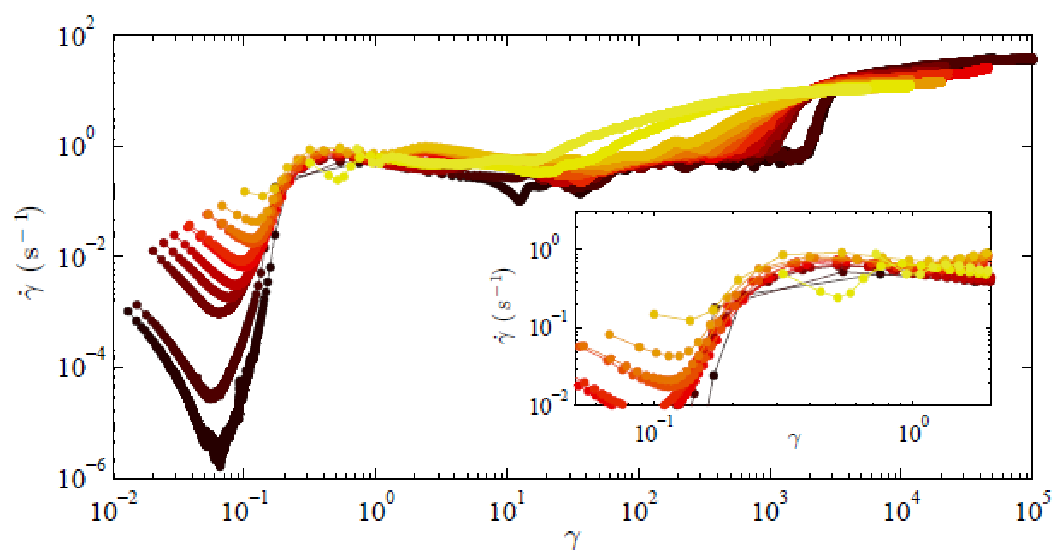
Figure 7: Creep experiments in an 8% w/w CB gel under rough boundary conditions. Shear rate responses \dot{\gamma} as a function of the strain \gamma for different shear stresses \sigma applied at time t = 0 : from right to left, \sigma = 24, 27, 35, 38, 41, 45, 47, 50, 52, 55, 60, 70, and 80 Pa. Inset: enlargement over the end of the initial creep regime.
