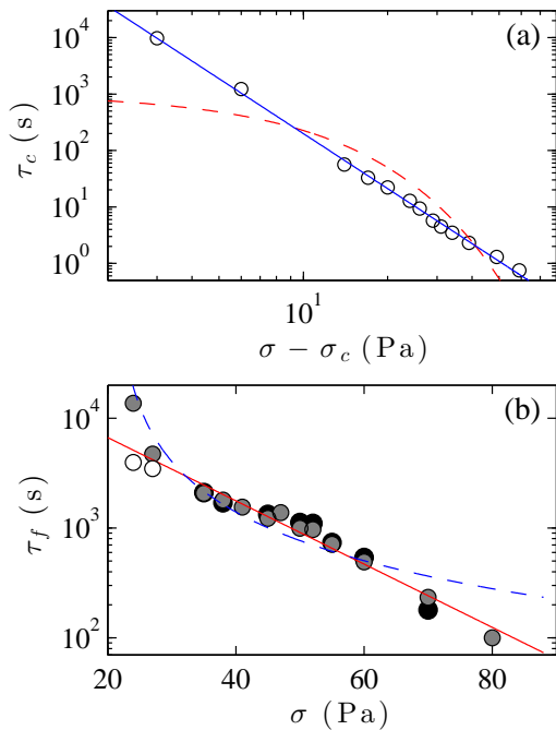
Figure 7: Characteristic timescales for yielding of an 8 % w/w CB gel under rough boundary conditions as a function of the imposed shear stress \sigma . (a) Duration of the creep regime \tau_c (or equivalently time at which total wall slip is observed) as a function of the reduced shear stress \sigma - \sigma_c with \sigma_c = 21.0 Pa in logarithmic scales. The blue line shows the best power-law fit \tau_c \sim (\sigma - \sigma_c)^{-\beta} with \beta = 3.2 \pm 0.1 . The red dashed line is the best exponential fit of \tau_c . (b) Full fluidization time \tau_f vs \sigma in semilogarithmic scales. Gray symbols correspond to estimations derived from rheological data while black symbols are times extracted from velocity measurements. White symbols show \tau_f - \tau_c for the two lowest stresses (where \tau_c > 0.2\tau_f ). The red line shows the best exponential fit \tau_f = \tau_0 \exp(-\sigma/\sigma_0) with \tau_0 = 2.6 \pm 0.1 10^4 s and \sigma_0 = 15.0 \pm 0.1 Pa when excluding the two leftmost points. The blue dashed line is the best power-law fit \tau_f \sim (\sigma - \sigma_c)^{-\beta} of the full data set with \sigma_c = 21.0 Pa. No satisfactory power-law fit of \tau_f can be found when allowing \sigma_c to vary.
