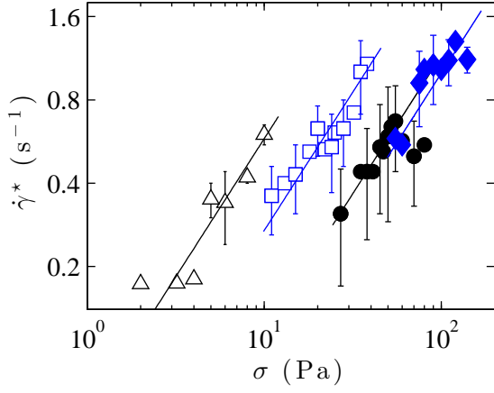
Figure 6: Shear rate \dot{\gamma}^* after failure at the inner wall at t = \tau_c as a function of the applied shear stress \sigma for CB gels of concentration C = 4 ( \triangle ), 6 ( \square ), 8 ( \bullet ), and 10% w/w ( \blacklozenge ). Solid lines correspond to linear behaviours \dot{\gamma}^* \propto \sigma . Error bars show the variations of \dot{\gamma}(t) over the shear rate plateau for \tau_c < t < \tau_f .
