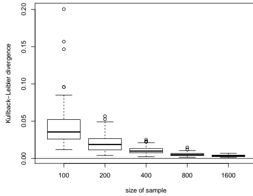
(b) Kullback-Leibler divergence from the true model
