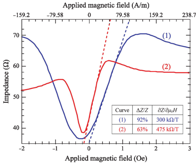
Fig. 1. Comparison between the modulus of the impedance as a function of the applied longitudinal field for a representative Co-rich amorphous wire operating at: (1) 30 MHz with a 10 mA dc bias current and (2) 3 MHz with a 2 mA dc bias current.
