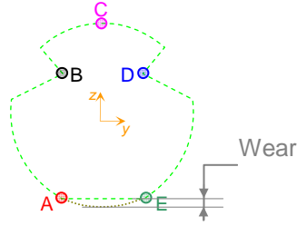
Figure 13. Virtual contact wire section.
