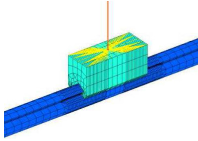
Figure 11. Dropper claw and boundary conditions.
