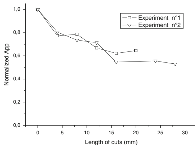
Fig. 10 Variation of the normalized peak-to-peak amplitude ( A_{pp} ) of the BKG signal (normalized to the signal intensity of the first measurement) after successive cuts of the nail sample. After each cut, the cut edges were humidified to eliminate MIS. For all measurements, the samples have the same geometry in the cavity. The experiment was performed twice. The measurements were performed at X-band
