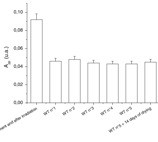
Fig. 22 Influence of humidity on the RIS5 intensity determined by multiple water treatment (WT). Measurements were performed at Q-band
