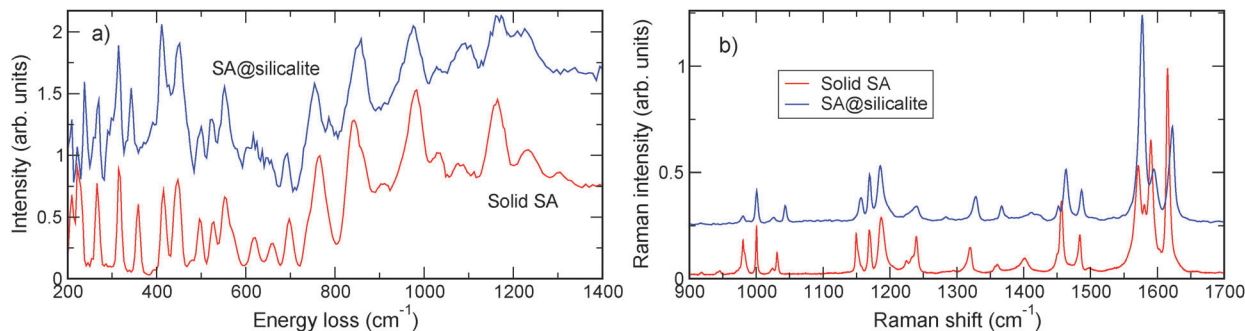
Fig. 7 INS (a) and Raman (b) spectra of the SA molecules sorbed in silicalite-1 (noted hereafter as SA@silicalite) compared with the spectra of the molecule in solid phase.
