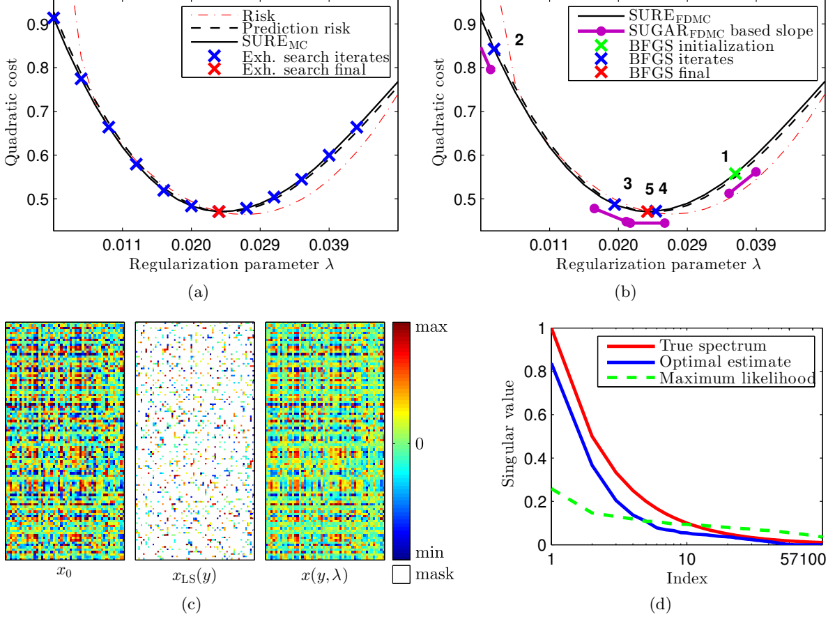
Figure 4: (a-b) Risk, prediction risk and its SURE estimates** as a function of the regularization parameter \lambda . (a) The 12 points where \text{SURE}_{\text{MC}}\{x\}(y, \lambda, \delta) has been evaluated by exhaustive search. (b) The 5 evaluation points of \text{SURE}_{\text{FDMC}}\{x\}(y, \lambda, \delta, \varepsilon) and \text{SUGAR}_{\text{FDMC}}\{x\}(y, \lambda, \delta, \varepsilon) required by BFGS to reach the optimal one. (c-d) Respectively, a close in and the spectrum of the underlying matrix x_0 , the least-square estimate x_{\text{LS}}(y) and the solution x(y, \lambda) at the optimal \lambda .
