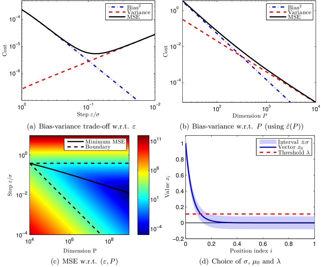
Figure 1: Bias-variance trade-off of the gradient estimator of the DOF of soft-thresholding, (a) with respect to the step \varepsilon and (b) with respect to the dimension P when using a power decay function P \mapsto \hat{\varepsilon}(P) . (c) Its mean squared error as a function of P and \varepsilon (in logarithmic scales). The solid line represents the pairs (\hat{\varepsilon}^*(P), P) where, for a fixed dimension P , \hat{\varepsilon}^*(P) minimizes the mean squared error. The function \hat{\varepsilon}^*(P) looks like a power function of the form of C\sigma/P^\alpha with C > 0 and 0 < \alpha < 1 . The dashed lines represent respectively the power functions \hat{\varepsilon}^{\text{inf}}(P) = C\sigma and \hat{\varepsilon}^{\text{sup}}(P) = C\sigma/P outside which the mean squared error diverges when P increases. (d) Description of the settings of the experiments, i.e., the choice of \sigma , \mu_0 and \lambda .
