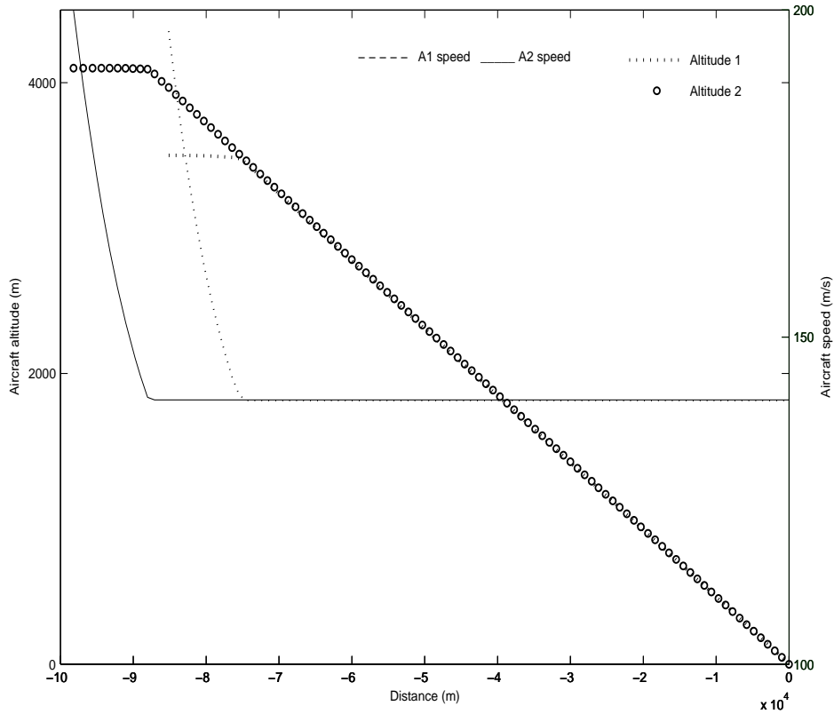
Figure 2: Aircraft optimal flight paths and speeds
