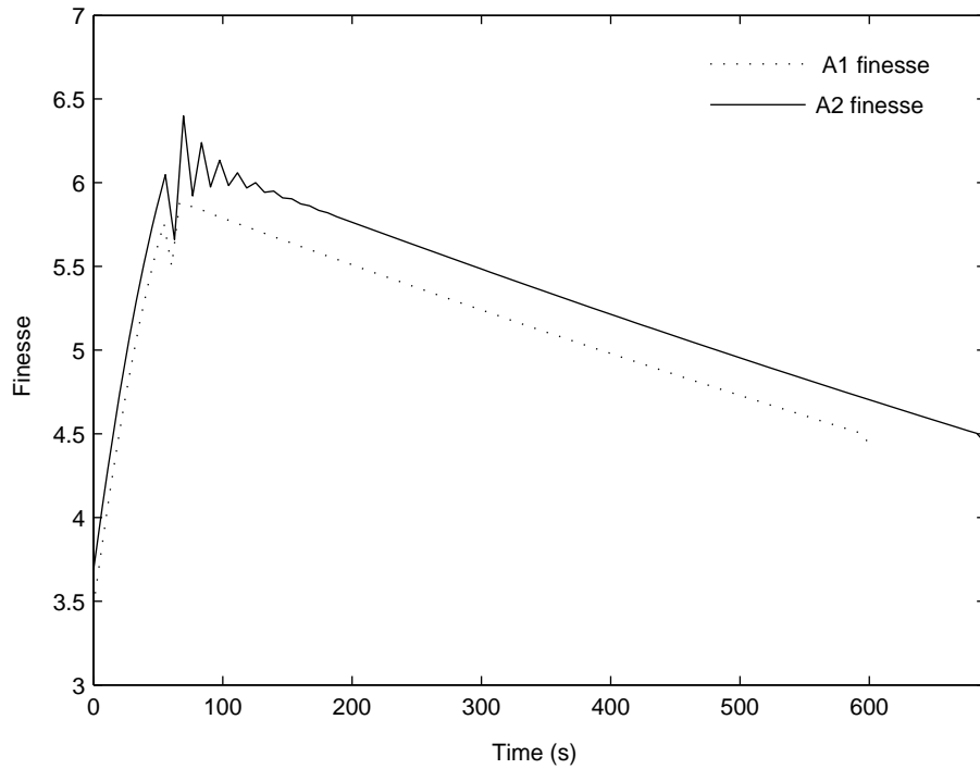
Figure 4: Aircraft finesse
