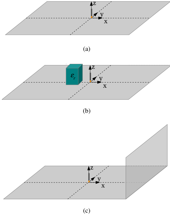
Fig. 2. (a) sub-case 1 : monopole on the square metallic plate; (b) sub-case 2 : monopole and dielectric block on the square metallic plate; (c) sub-case 3 : monopole mounted on the metallic dihedral structure.
