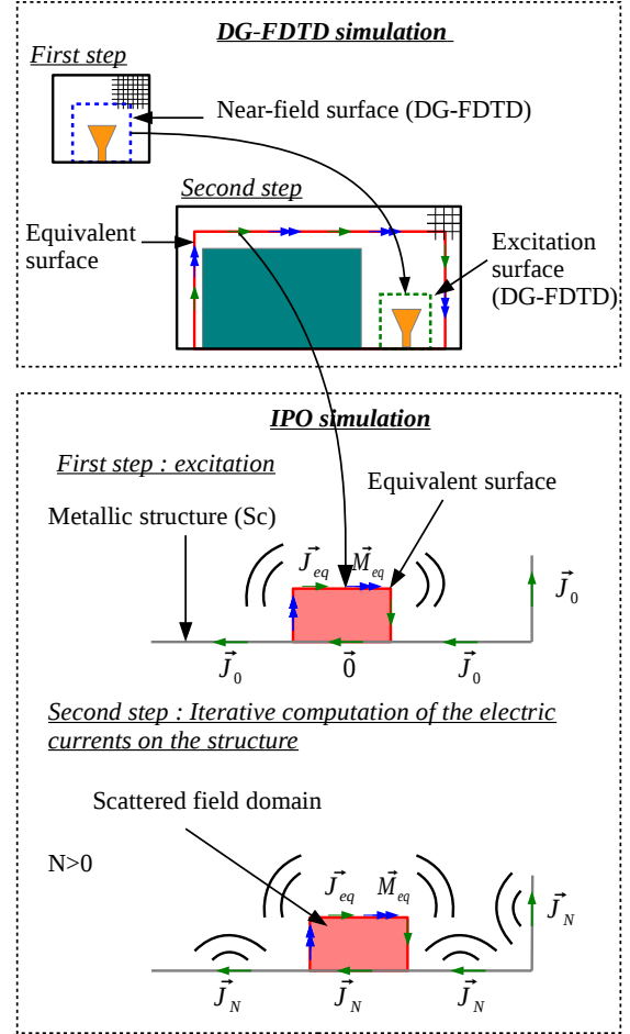
Fig. 3. DG-FDTD/IPO decomposition of the complete scenario.
