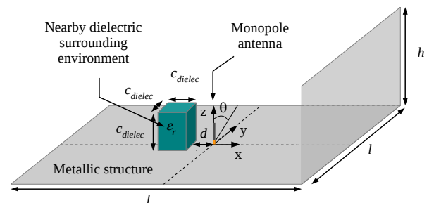
Fig. 1. Antenna mounted on a metallic structure. l = 3.9 \text{ m} = 13 \lambda_{1\text{GHz}} , h = 1.15 \text{ m} = 3.83 \lambda_{1\text{GHz}} , d = 0.15 \text{ m} = 0.5 \lambda_{1\text{GHz}} , C_{\text{dielec}} = 0.18 \text{ m} = 0.6 \lambda_{1\text{GHz}} , \epsilon_r = 10
