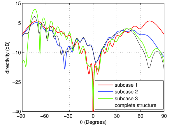
Fig. 4. Far-field results ( E_\theta ) in the (x0z) plane at 1 GHz.
