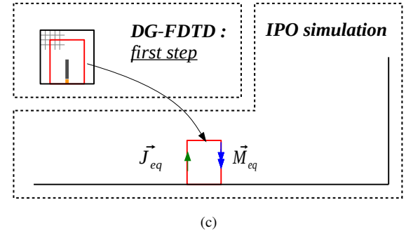
Fig. 6. Decomposition schemes used to simulate the sub-cases : (a) sub-case 1; (b) sub-case 2; (c) sub-case 3.
