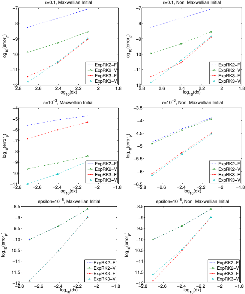
Figure 7.2. L_1 error for the density \rho for different exponential schemes. From the top to the bottom, results show \epsilon = 0.1, 10^{-3}, 10^{-6} respectively. Left column equilibrium initial data, right column non equilibrium initial data.
