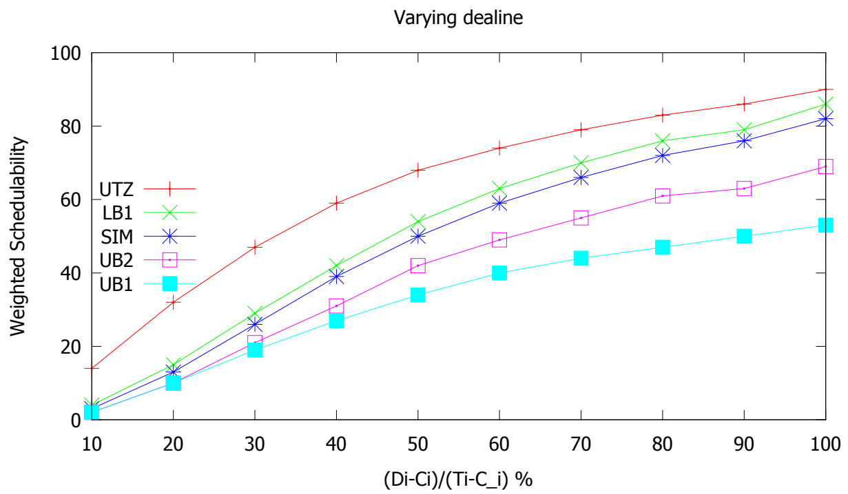
Figure 6: Varying relative deadlines in [C_i, T_i]
