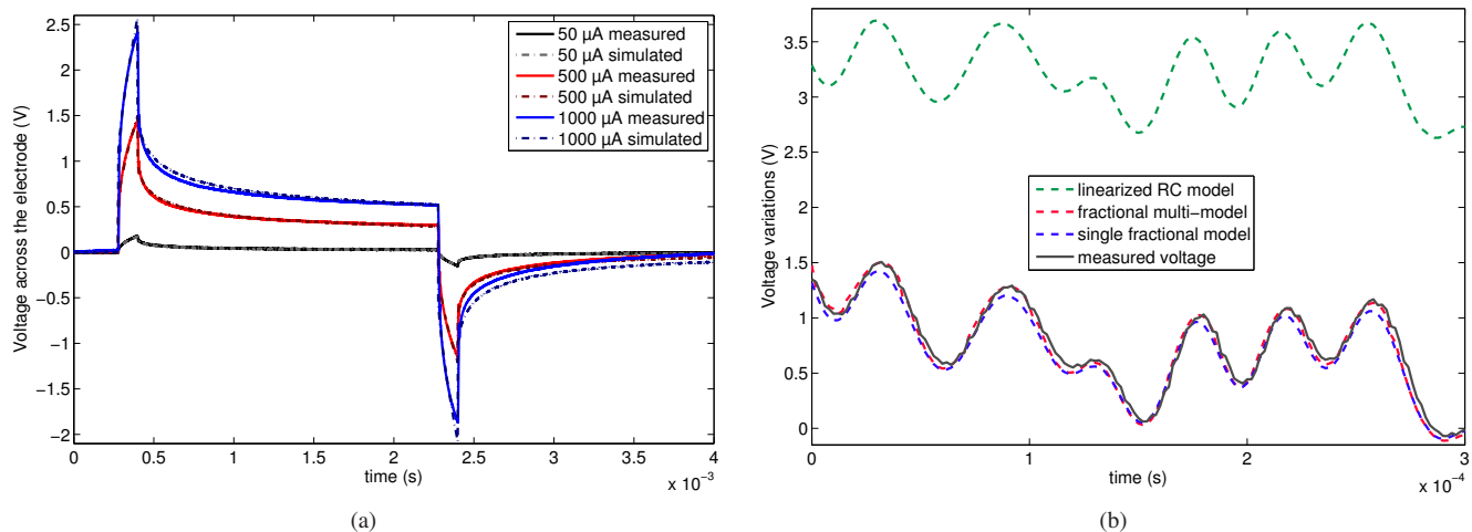
Fig. 3. 3(a) Comparison of measured step responses and simulated waveforms extracted from local models, 3(b) Comparison of voltage response to a pseudo-random current sequence obtained by measurement, fractional multi-model, single fractional model and linearized model.
