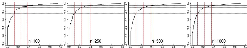
Figure 10: From left to right, the CDF for n = 100, 250, 500 and 1000 of the THO complexity in plain line using Algorithm 1. The horizontal black dotted lines provide the values 0.75, 0.9 and 0.95 and the vertical red dotted lines their respective quantiles.
