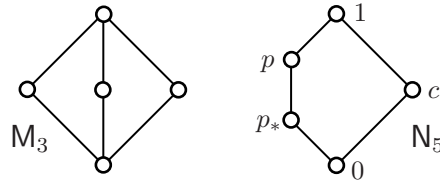
FIGURE 2.1. The lattices \mathbf{M}_3 and \mathbf{N}_5
