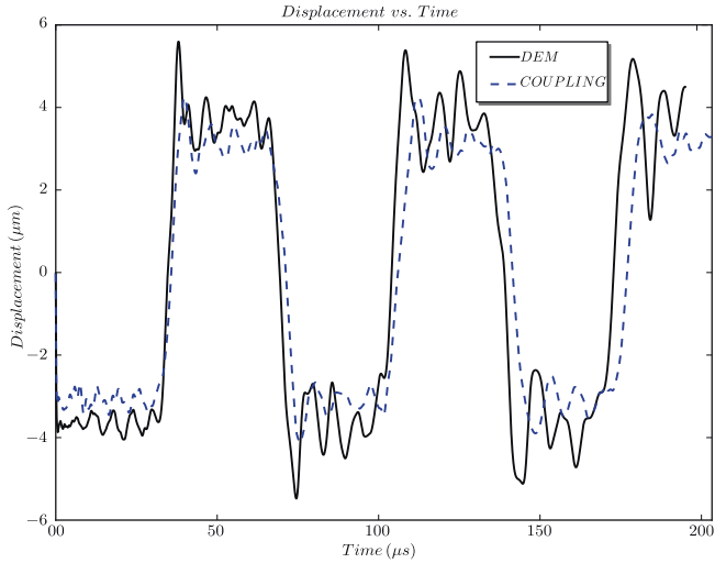
Fig. 22. Test4: The free-end displacement U_{x \text{ mean}} obtained by DEM and the coupling method L_0 = 10 mm, coarse multiplier space, continuous differentiable weight functions, \varepsilon = 0.05 .
