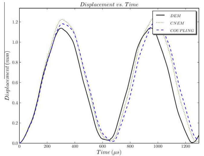
Fig. 20. Test2: The free-end displacements U_{y, mean} obtained by DEM, CNEM and the coupling method L_0 = 10 mm, coarse multiplier space, continuous differentiable weighting, \varepsilon = 0.05 .
