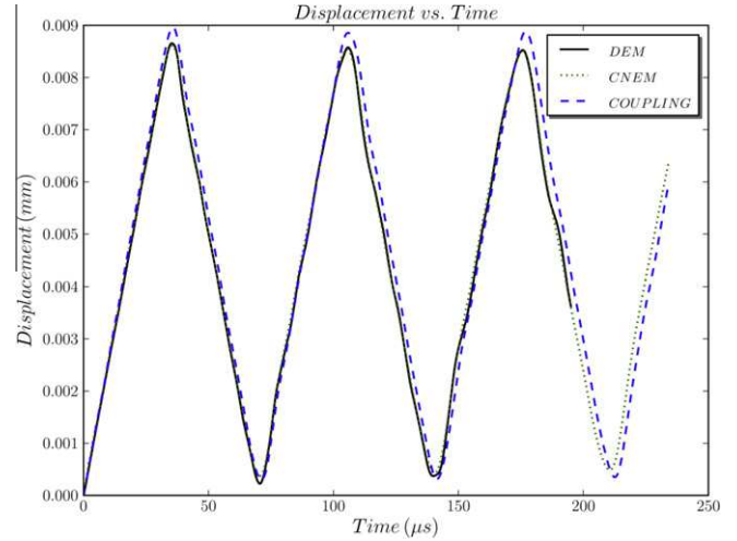
Fig. 19. Test1: The free-end displacements U_{x, mean} obtained by DEM, CNEM and the coupling method L_0 = 10 mm, coarse multiplier space, continuous differentiable weighting, \varepsilon = 0.05 .
