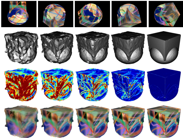
Figure 3. Evolution of the minimization at different iterations on a synthetic data (24 images of 640 \times 480 ). From top to bottom: 5 of the input images; 3D triangular mesh X ; Photometric reprojection error; Textured mesh using the estimated texture T .
