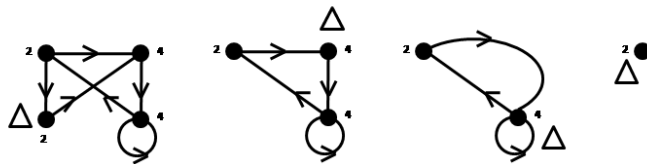
FIGURE 2. Playing DIRECTED VERTEXNIM
