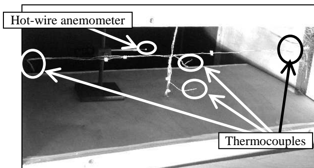
Figure 5: Picture of the sensors installed in the downstream section
