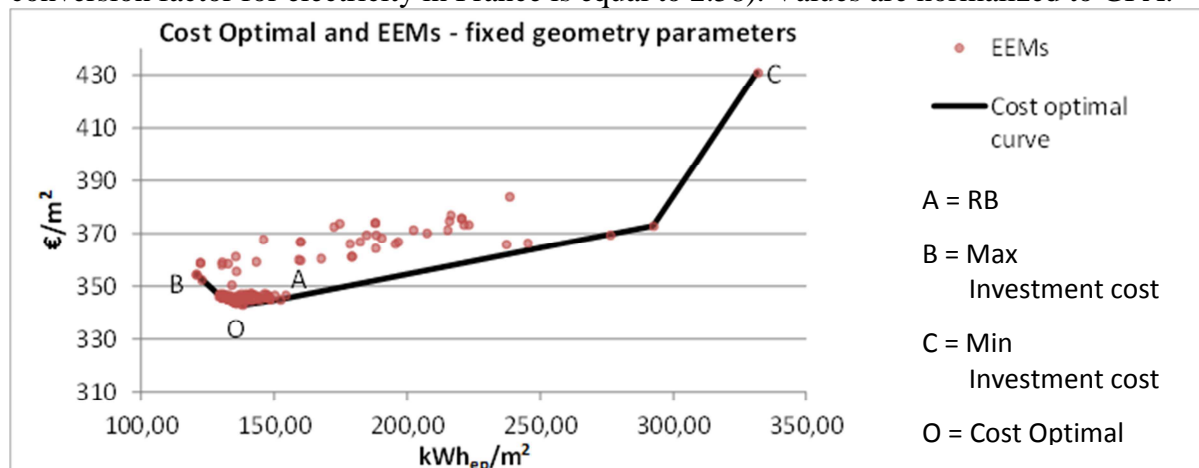
Figure 8. Cost optimal curve for RB geometry
