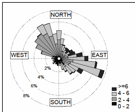
Fig. 7: Measured wind rose
