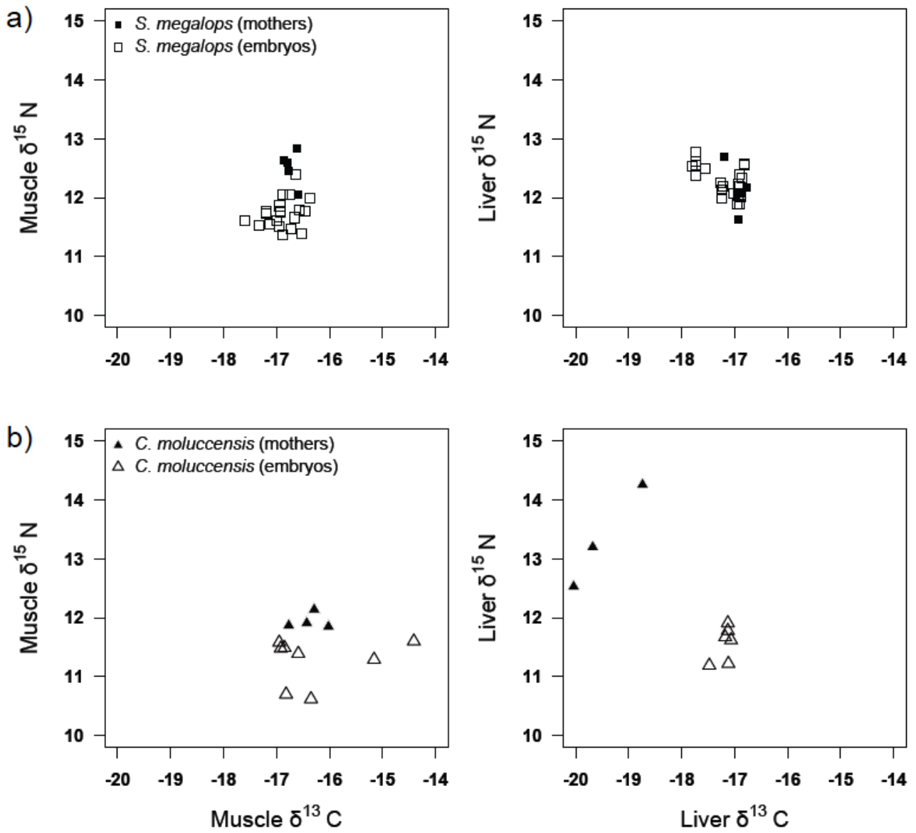
Fig. 1. Isotopic values (‰) from muscle and liver tissues in mothers and embryos of a) S. megalops and b) C. moluccensis .
