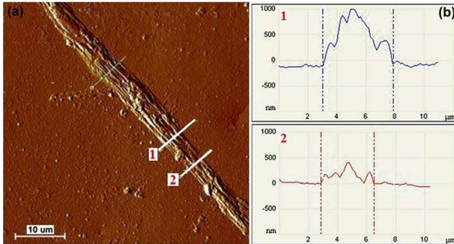
Fig. 9. Surface roughness of a type II persistent slip marking at stress amplitude of 57.5 MPa – N = 10^7 cycles – (a) AFM image and (b) surface profiles along the white lines numbered 1 and 2.
