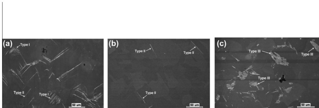
Fig. 12. SEM images of slip band formed at (a) stress amplitude of 90 MPa – N = 5 \times 10^5 cycles, (b) stress amplitude of 65 MPa – N = 10^6 cycles and (c) stress amplitude of 44 MPa – N = 4.5 \times 10^8 cycles.
