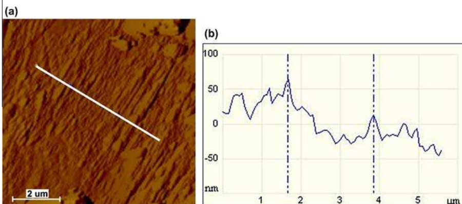
Fig. 11. Surface roughness of type III persistent slip markings at stress amplitude of 50 MPa – N = 2 \times 10^8 – (a) AFM image, and (b) surface profile along the white line.
