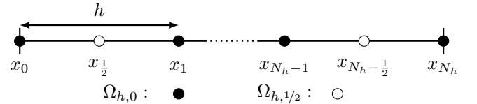
FIGURE 2 – Discrétisation spatiale
