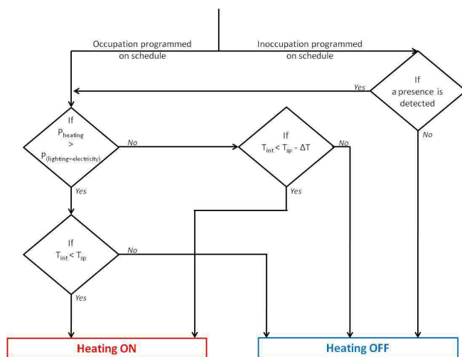
Fig. 6. Algorithm for heating strategy
