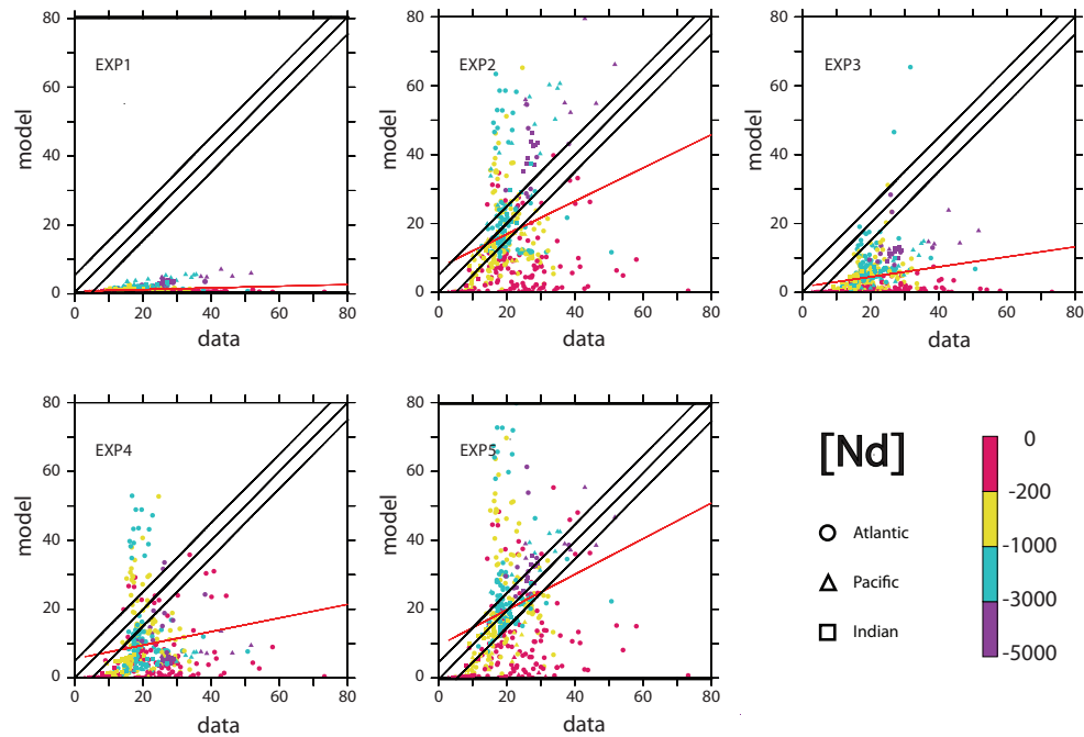
Fig. 6. Same figure as Fig. 4, for Nd concentration (in pmol/kg). Black lines represent the lines [\text{Nd}] (model)=[Nd] (data) and [\text{Nd}] (model)=[Nd] (data) \pm 10 pmol/kg, which represents a characteristic value used to define a good agreement between the model and the data.
