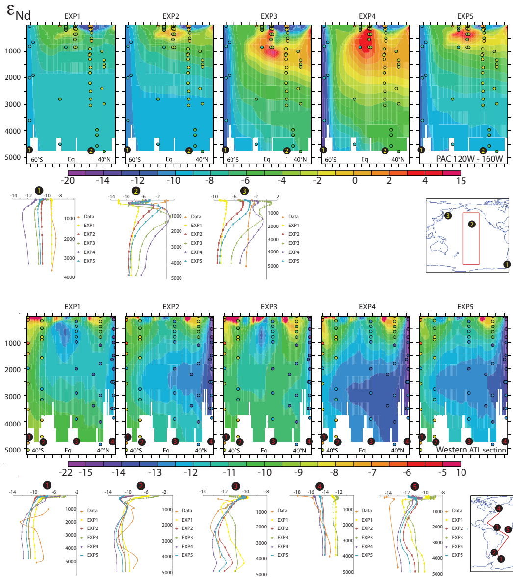
Fig. 3. Vertical \varepsilon_{\text{Nd}} sections for all simulations, in the Pacific basin averaged between 120^{\circ}\text{W} and 160^{\circ}\text{W} (upper panel), and along the western section of the Atlantic basin (lower panel). Superimposed circles are the data from the compilation by F. Lacan and T. van de Fliedert; http://www.legos.obs-mip.fr/fr/equipes/geomar/results/database_may06.xls (Piepgras et Wasserburg, 1982; Piepgras et Wasserburg, 1983; Stordal et Wasserburg, 1986; Piepgras et Wasserburg, 1987; Piepgras et Jacobsen, 1989; Jeandel, 1993; Jeandel et al., 1998; Lacan et Jeandel, 2001, Amakawa et al., 2004). Colour scales are the same for all simulations and data, but different for each section. For each basin, characteristic profiles are numbered and located on the associated map, and at the bottom of each transect, for each experiment. Main characteristics for each experiment are summarized in Table 1.
